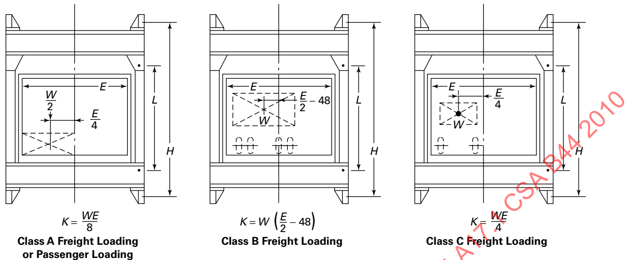
Fig. 8.2.2.5.1 Turning Moment Based on Class of Loading
