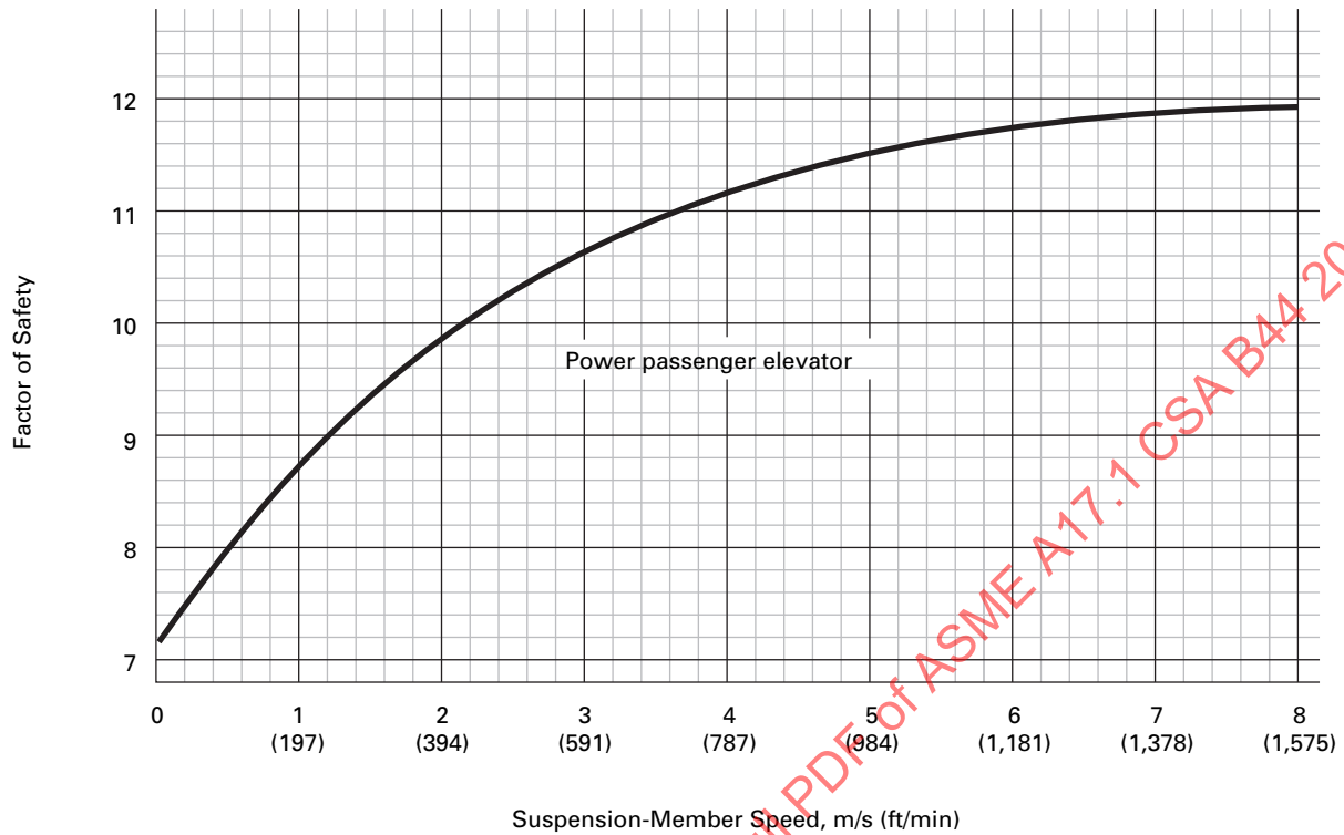
(10) Fig. 8.2.7 Minimum Factors of Safety of Suspension Members of Power Passenger and Freight Elevators
