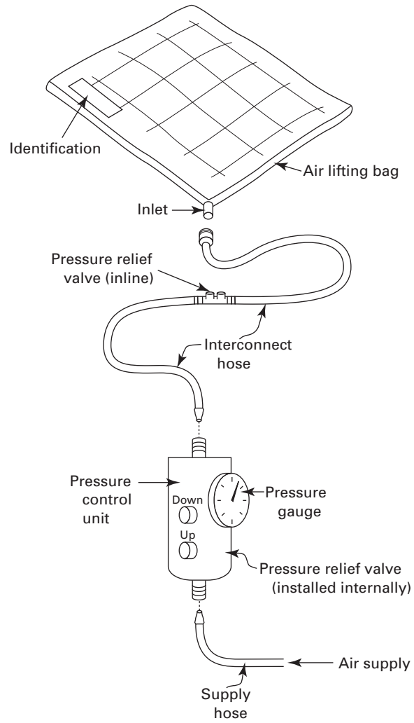
Fig. 1-3.1.1-1 Air-Lifting Bags
