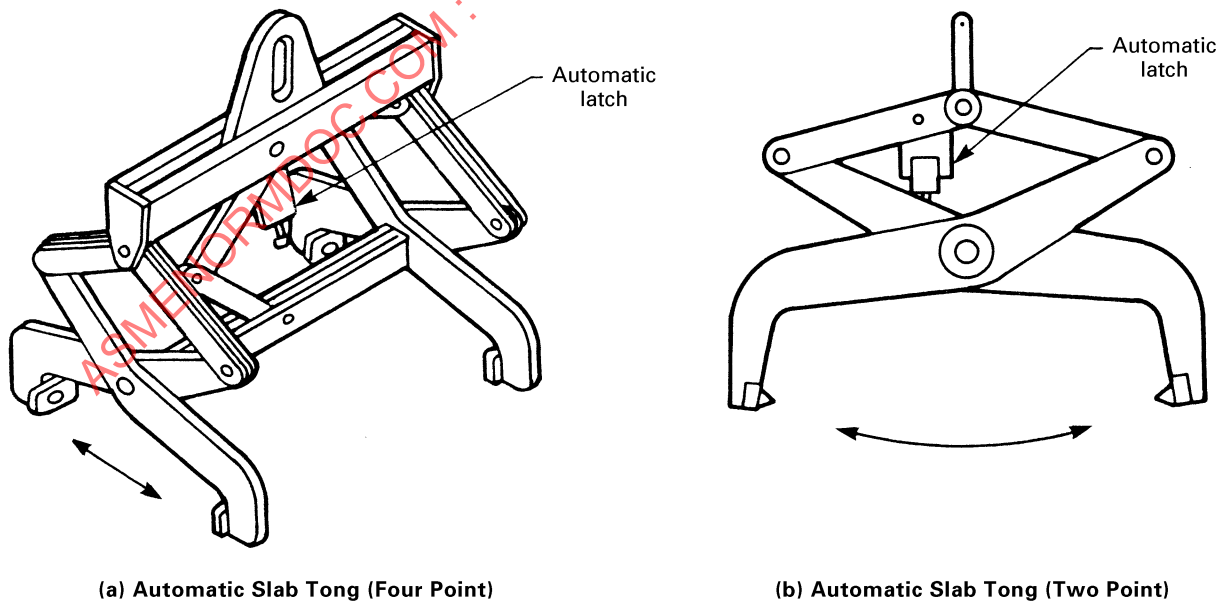
Fig. 20-0.3-3 Pressure-Gripping Lifters: Indentation-Type Lifters
