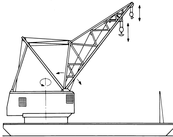
Fig. 8-0.1-1 Floating Crane
