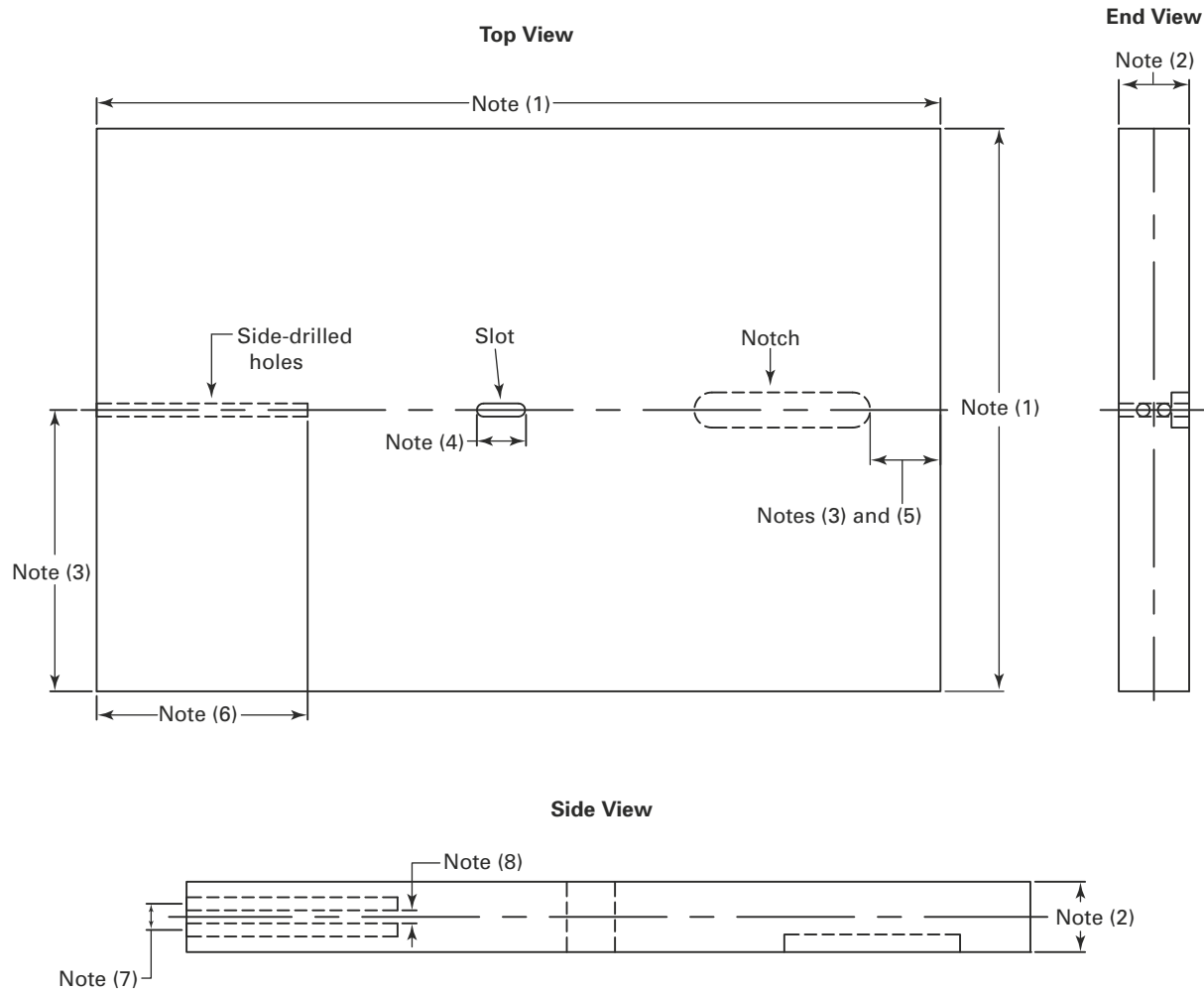
Figure T-334.1-1 Calibration Block
