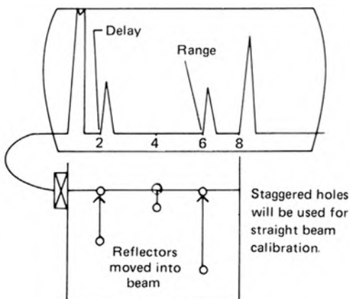
Figure C-461 Sweep Range
