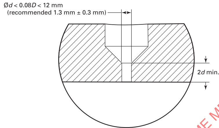
Fig. 7.5-1 Pressure Tap Schematic
