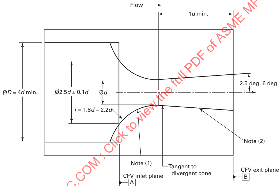
Fig. 6.2.1-1 Toroidal Throat CFV Geometry
