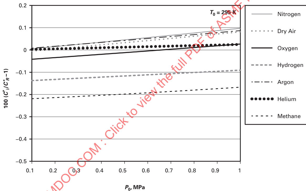
Fig. 8.2-2 Percent Difference Between the Polytropic Gas Critical Flow Function, C_p^* , and the Real Gas Critical Flow Function, C_R^* , at T_0 = 295 K
