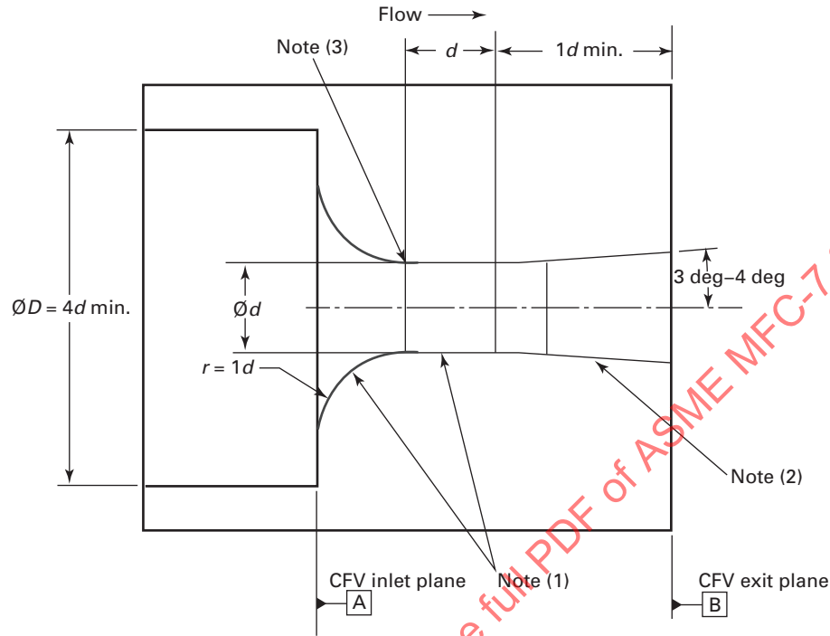
Fig. 6.2.2-1 Cylindrical Throat CFV Geometry
