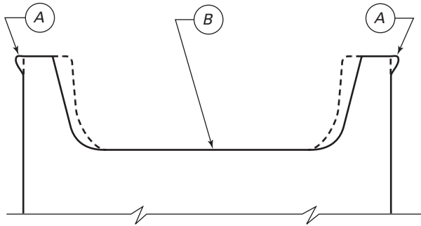
Fig. 7521.2-1 Inspection for Wheel Wear
