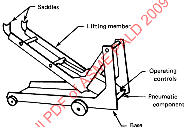
Fig. 10-1 Typical Swing-Type Mobile Lift
