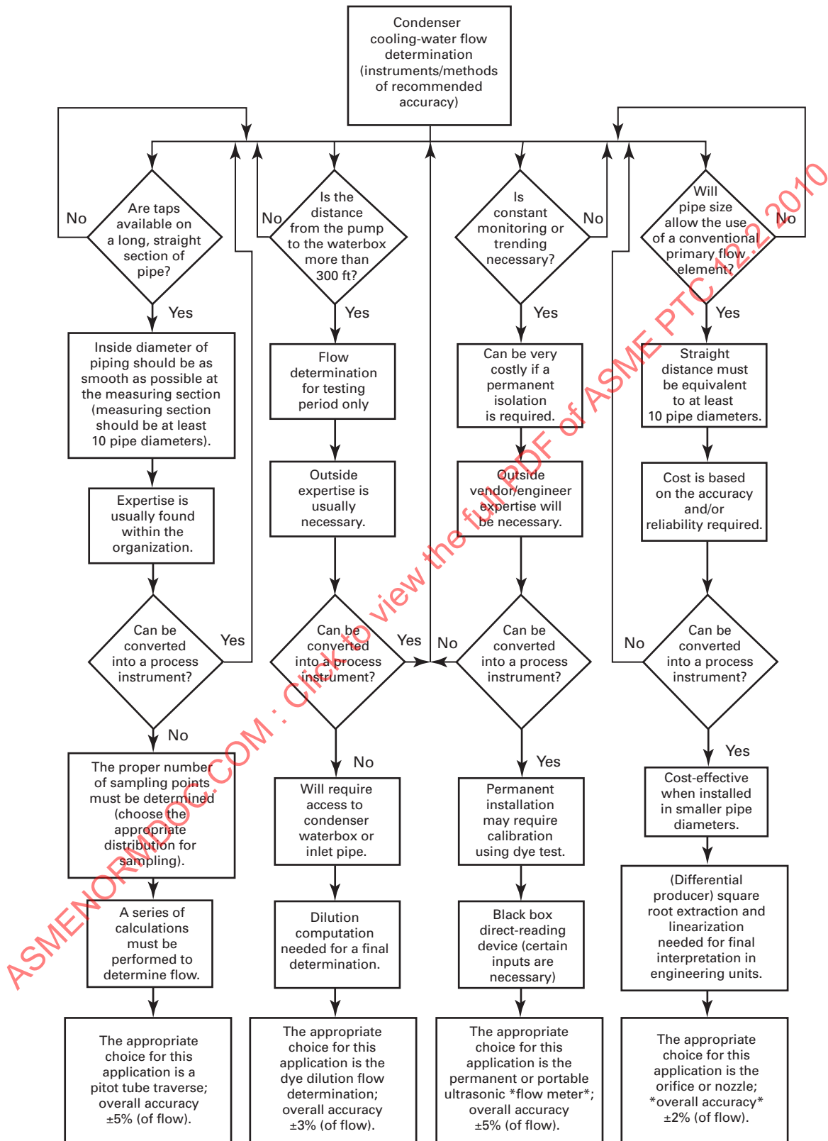
Fig. B-2 Selection of Measurement Devices for Cooling-Water Flow
