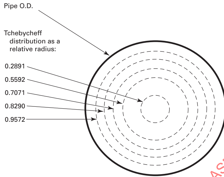
(a) 10-Point Traverse (I.D. ≤ 24 in.)
