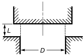
Flat-Seated Valve
