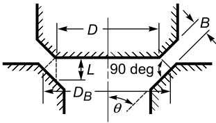
Bevel-Seated Valve
