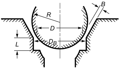
Radial-Seated Valve
