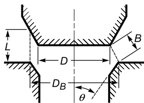
Bevel-Seated Valve
