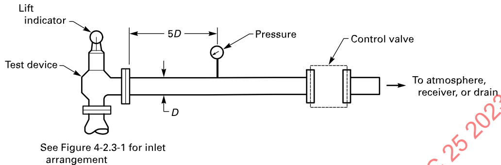
Figure 4-6.1-1 Recommended Discharge Arrangement for Testing Devices With Built-Up Back Pressure
