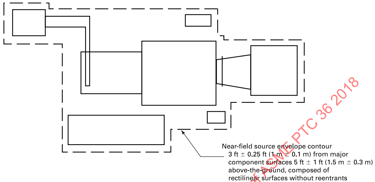
Figure 4-3.2.3-1 Near-Field Contours
