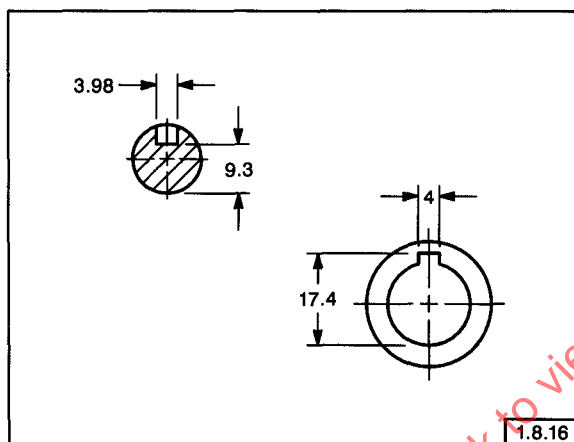
FIG. 1-45 KEYSEATS
