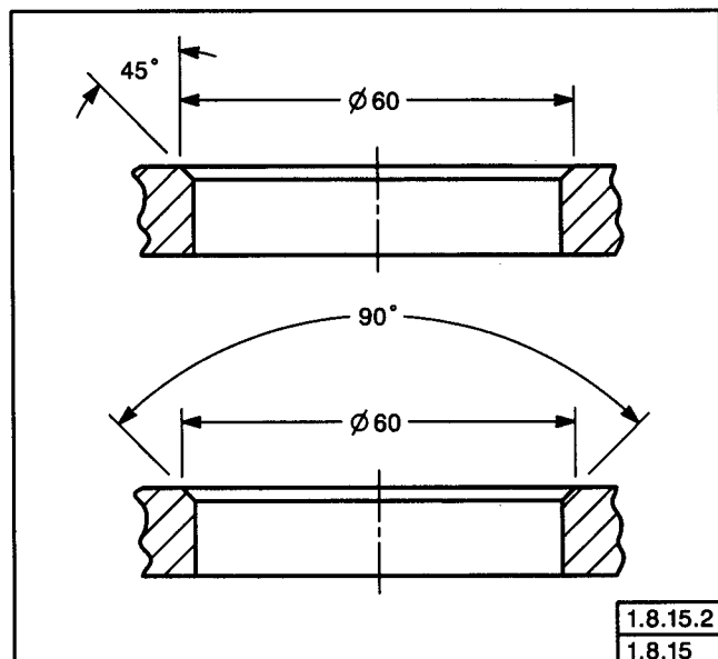
FIG. 1-43 INTERNAL CHAMFERS
