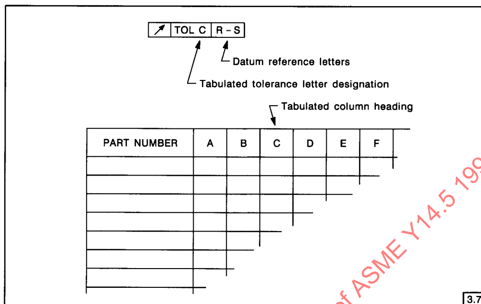
FIG. 3-26 TABULATED TOLERANCES
