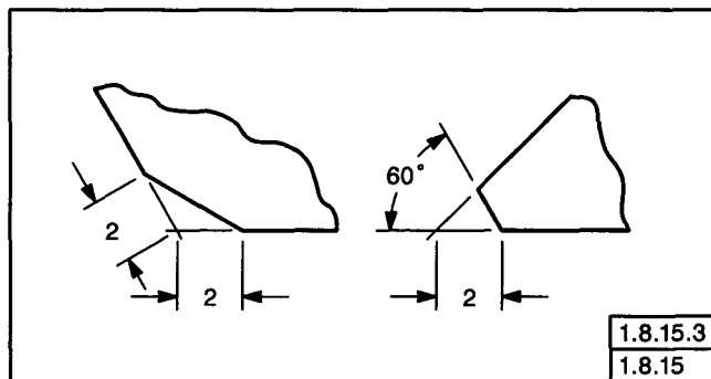
FIG. 1-44 CHAMFERS BETWEEN SURFACES AT OTHER THAN 90 DEGREES
