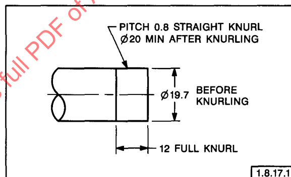
FIG. 1-47 KNURLS FOR PRESS FITS
