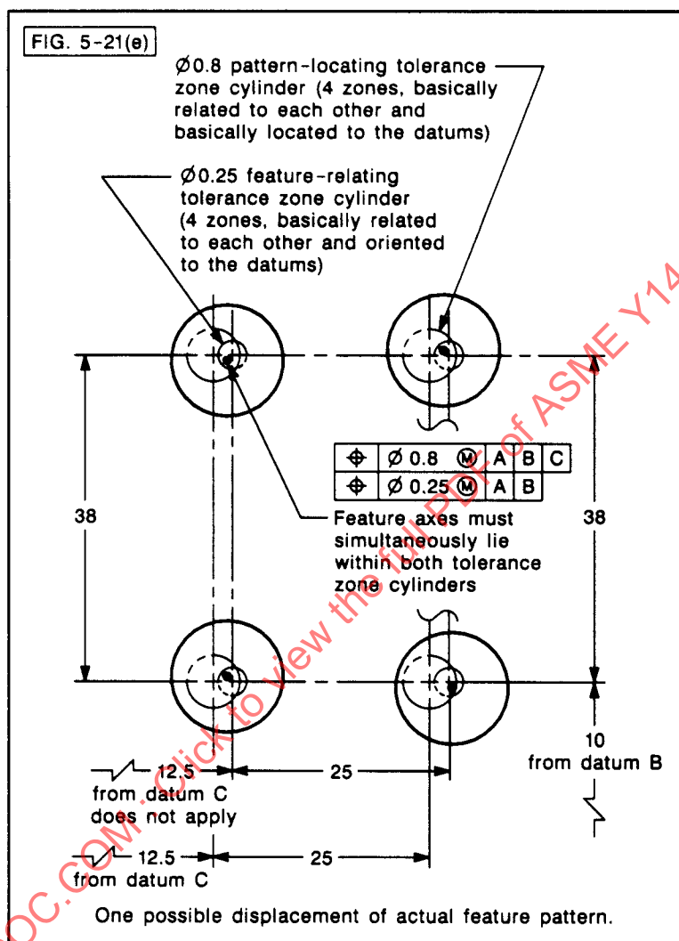
FIG. 5-21 HOLE PATTERNS OF FIG. 5-19. TWO SINGLE-SEGMENT FEATURE CONTROL FRAMES WITH SECONDARY DATUM IN LOWER FEATURE CONTROL FRAME (CONT'D) Tolerance Zones for Four-Hole Pattern
