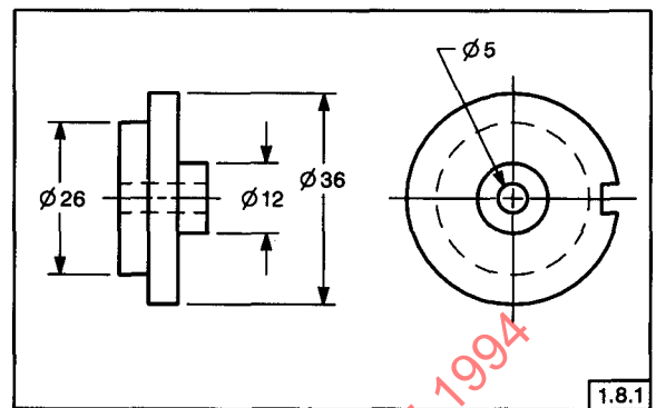
FIG. 1-19 DIAMETERS
