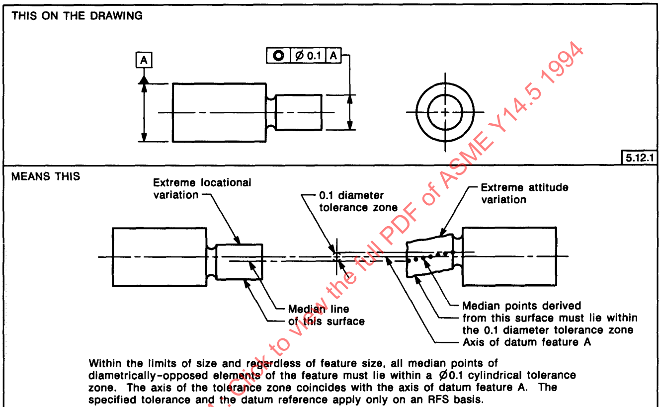
FIG. 5-54 CONCENTRICITY TOLERANCING
