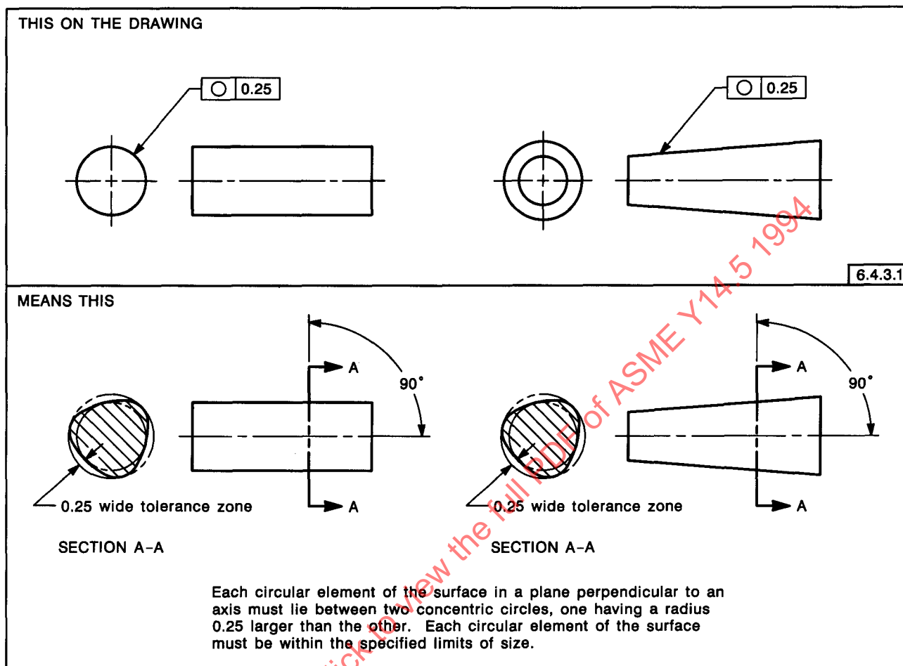
FIG. 6-8 SPECIFYING CIRCULARITY FOR A CYLINDER OR CONE
