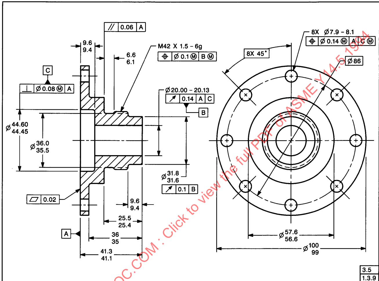
FIG. 3-25 FEATURE CONTROL FRAME PLACEMENT
