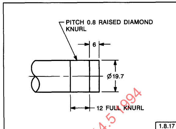
FIG. 1-46 KNURLS
