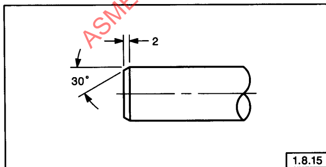
FIG. 1-41 CHAMFERS
