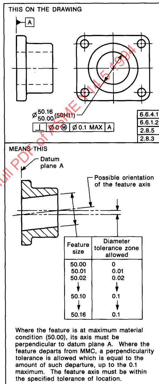
FIG. 6-42 SPECIFYING PERPENDICULARITY FOR AN AXIS (ZERO TOLERANCE AT MMC WITH A MAXIMUM SPECIFIED)
