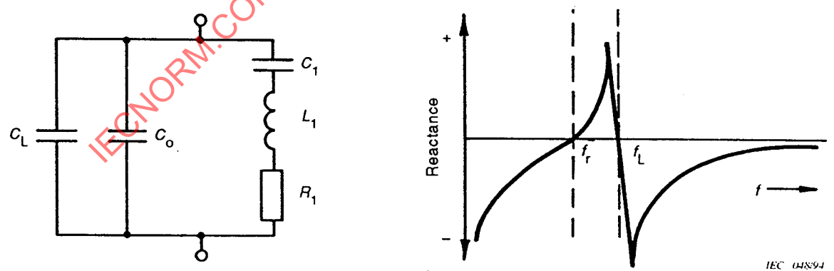
Figure 13c – Piezoelectric ceramic resonator unit with a parallel connected load capacitance C_L
