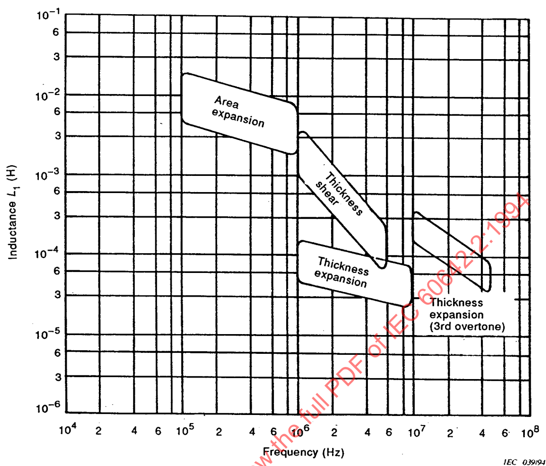
Figure 6 – Inductance ranges for various modes of vibration
