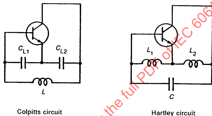
Figure 15 – Basic configuration of LC-oscillation circuit
