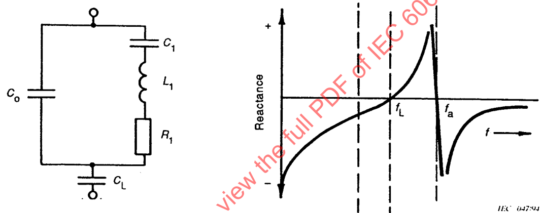
Figure 13b – Piezoelectric ceramic resonator unit with a series connected load capacitance C_L
