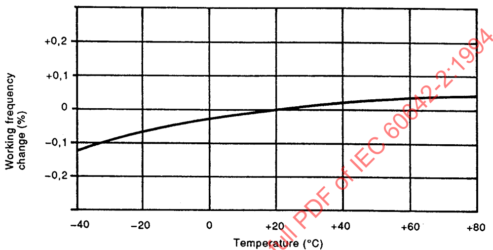
Figure 12 – A typical frequency versus temperature characteristic of working frequency with a piezoelectric ceramic resonator unit
