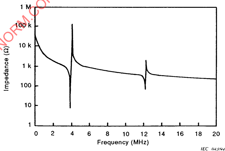
Figure 10 – A typical impedance characteristic of a thickness shear mode piezoelectric ceramic resonator
