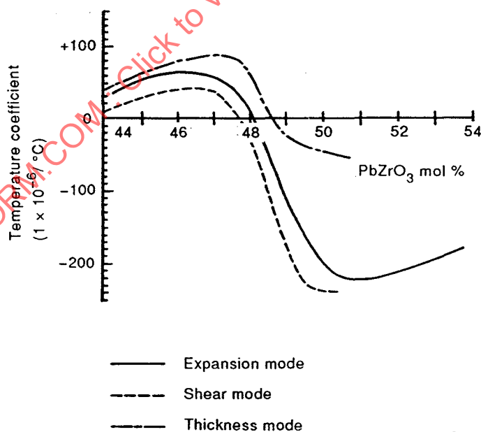
Figure 5 – Temperature coefficient characteristics of resonance frequency by \text{PbZrO}_3 ratio to \text{PbTiO}_3
