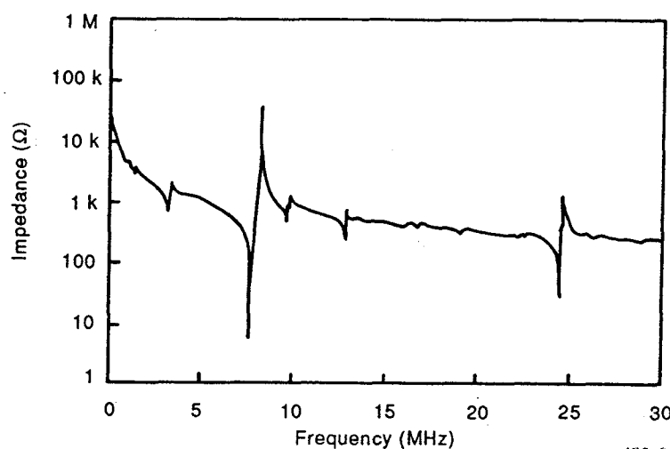
Figure 11 – A typical impedance characteristic of a thickness expansion mode piezoelectric ceramic resonator
