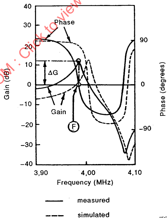
Figure 18 – Gain-phase characteristics showing actual measurements and computer simulation
