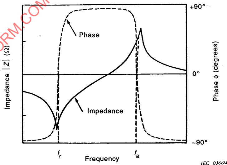
Figure 3 – Impedance and phase variation characteristics by frequency in the vicinity of resonance
