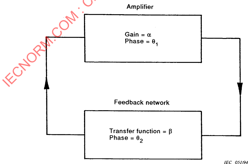
Figure 16 – Operating principle of an oscillation circuit
