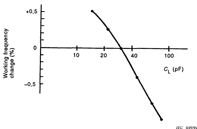
Figure 14 – An example of working frequency change due to a parallel connected load capacitance C_L
