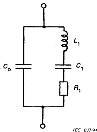
Figure 4 – Simplified equivalent circuit of a piezoelectric ceramic resonator
