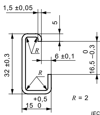
Figure A.9 – Dimensions of "G" section rails
