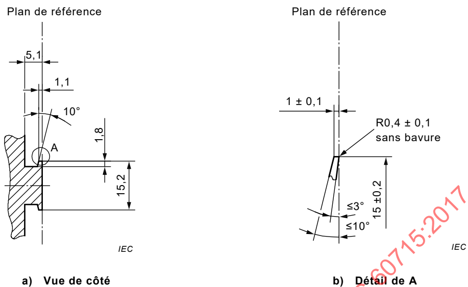
Figure 1 – Profilé-support TH 15
