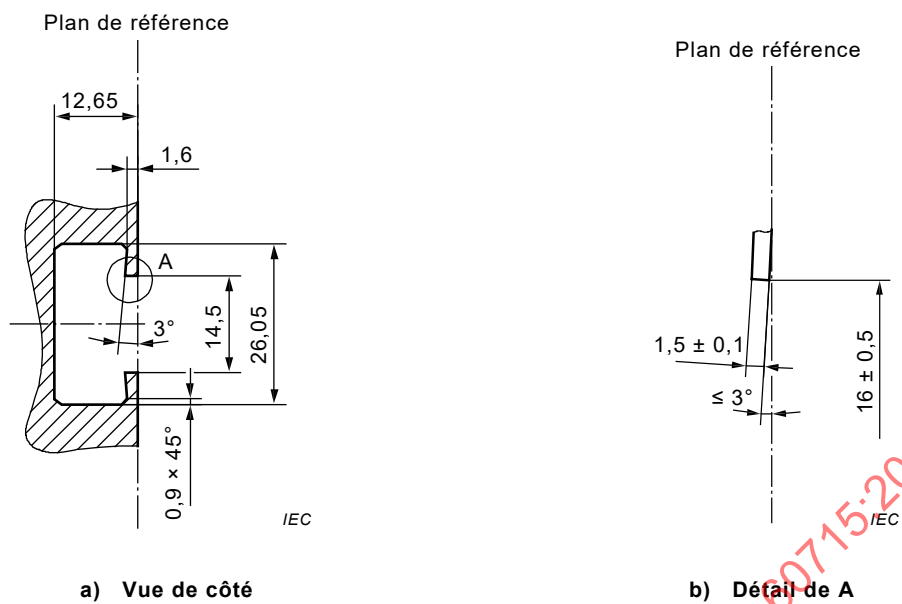
Figure 5 – Profilé-support C 30
