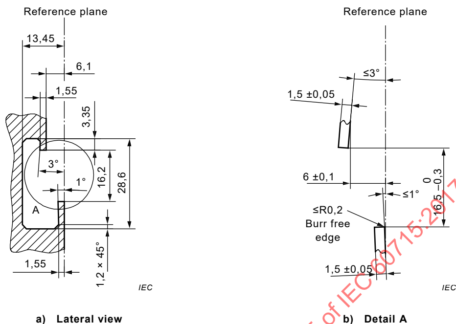
Figure 8 – Mounting rail G 32
