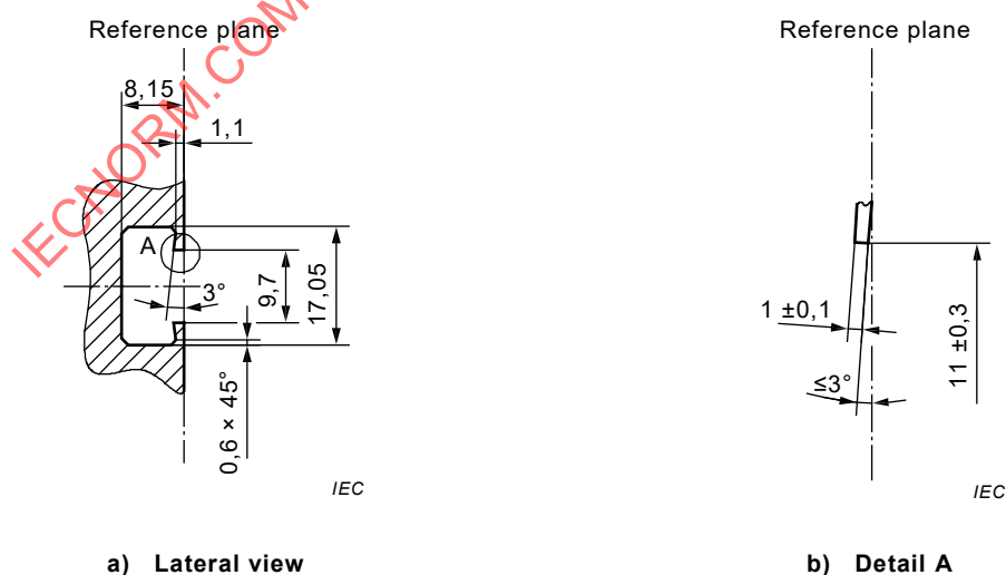
Figure 4 – Mounting rail C 20
