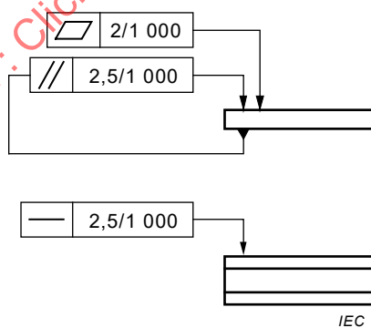
Figure A.8 – Tolerances (C 20, C 30, C 40 and C 50)
