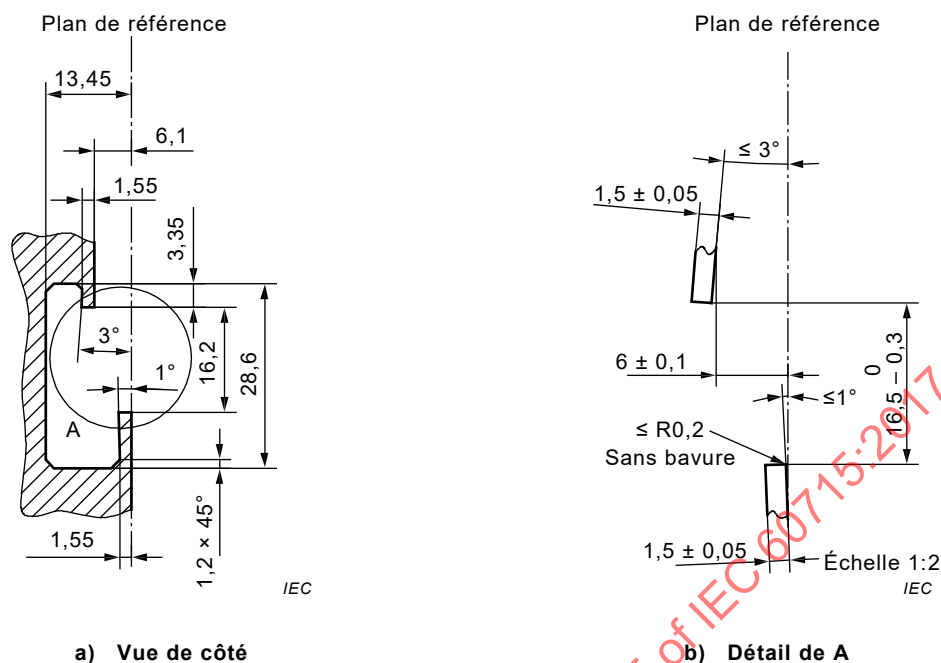
Figure 8 – Profilé-support G 32
