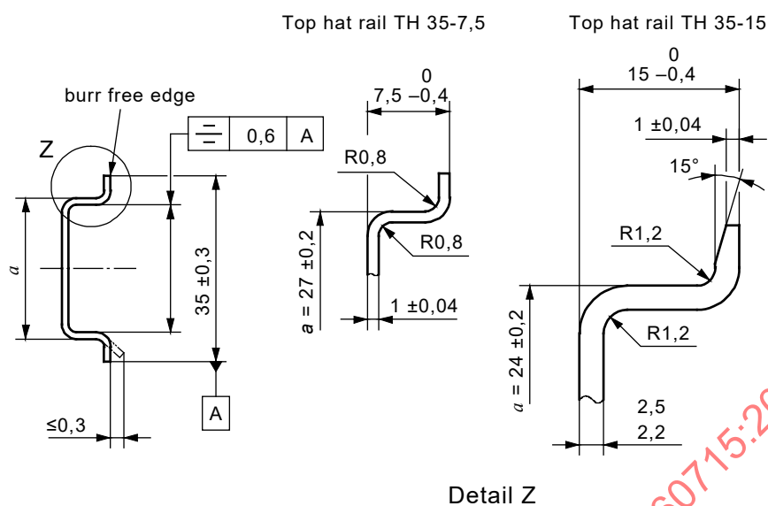
Figure A.3 – Top hat rails 35 mm wide for snap-on mounting of equipment
