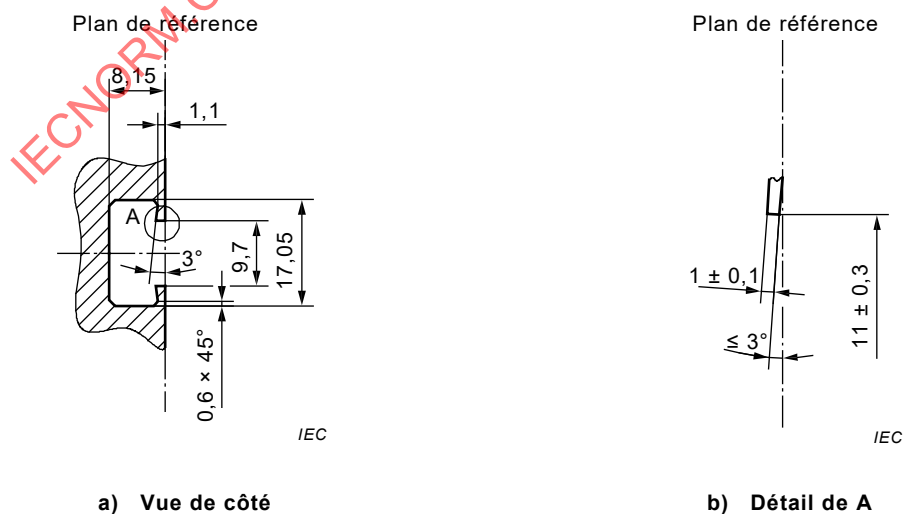
Figure 4 – Profilé-support C 20
