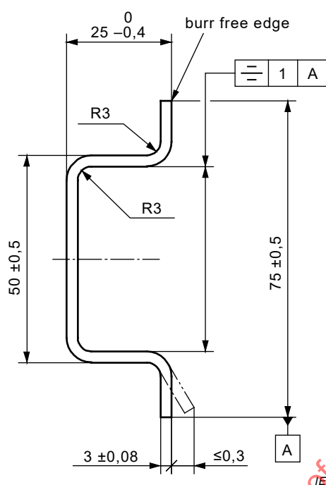
Figure A.5 – Top hat rail 75 mm wide for snap-on mounting of equipment
