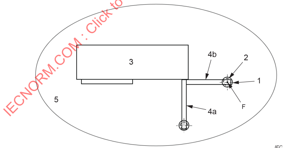
Figure 4 – Apparatus for load applied to a street cabinet door – Front view
