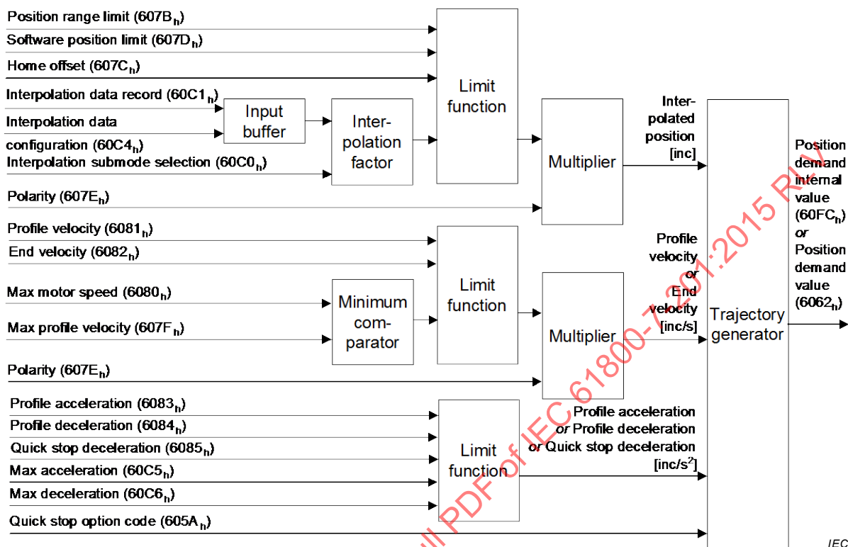
Figure 48 – Interpolation controller
