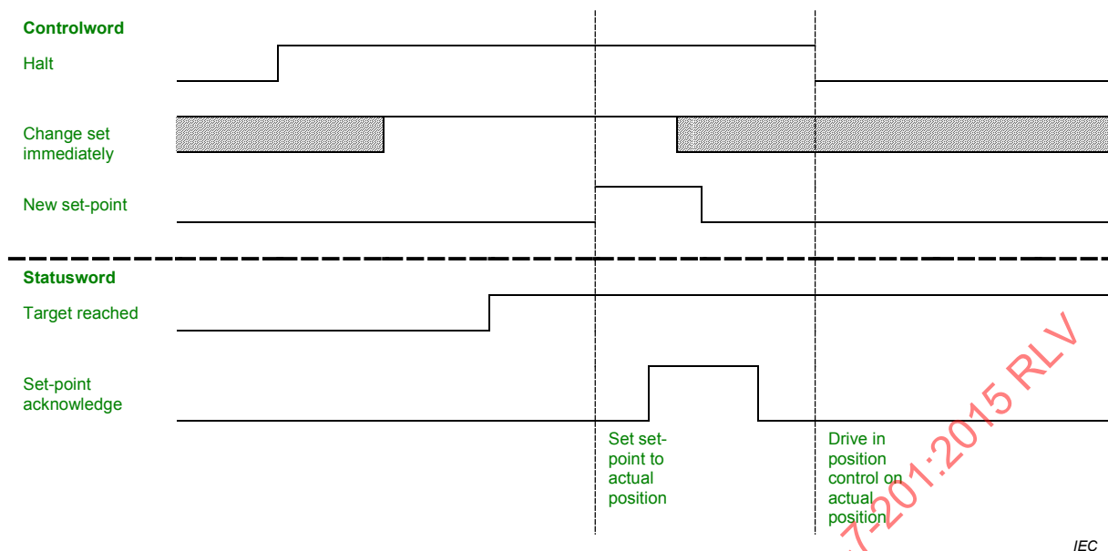
Figure 21 – Erase set-point
