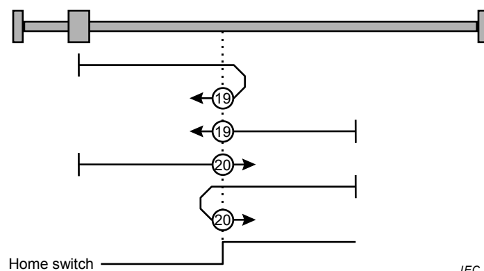
Figure 33 – Homing on positive home switch
