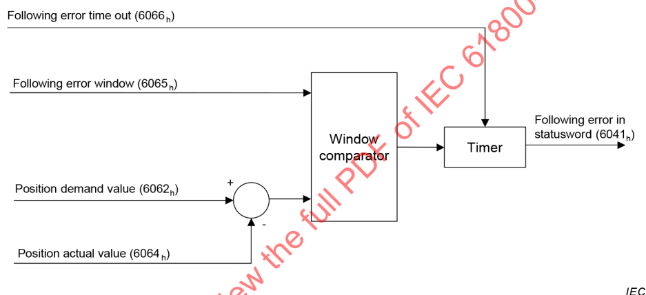
Figure 40 – Following error (functional overview)
