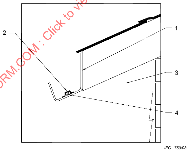
Figure 12 – Roof and gutter trace heater arrangement
