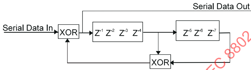
Figure 89—Data scrambler
