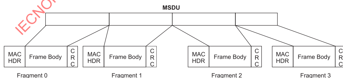
Figure 48—Fragmentation
