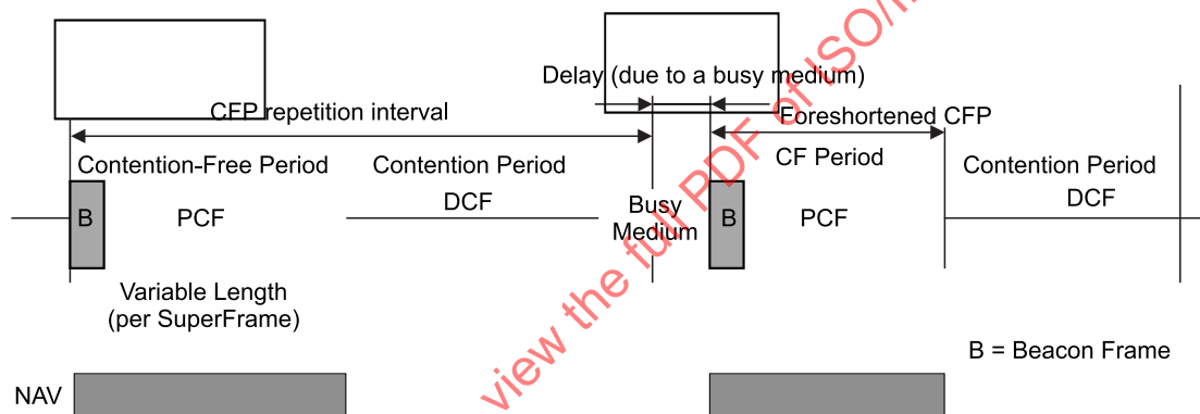
Figure 59—CFP/CP alternation
