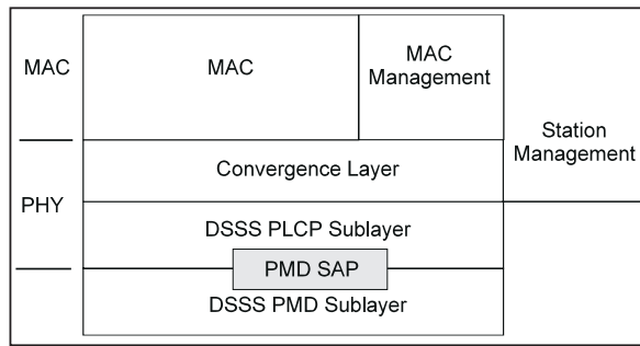
Figure 95—PMD layer reference model
