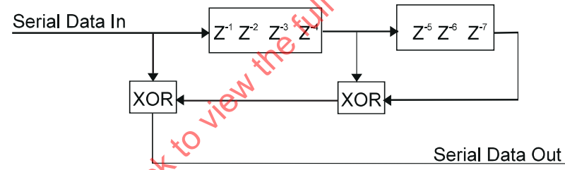
Figure 90—Data descrambler
