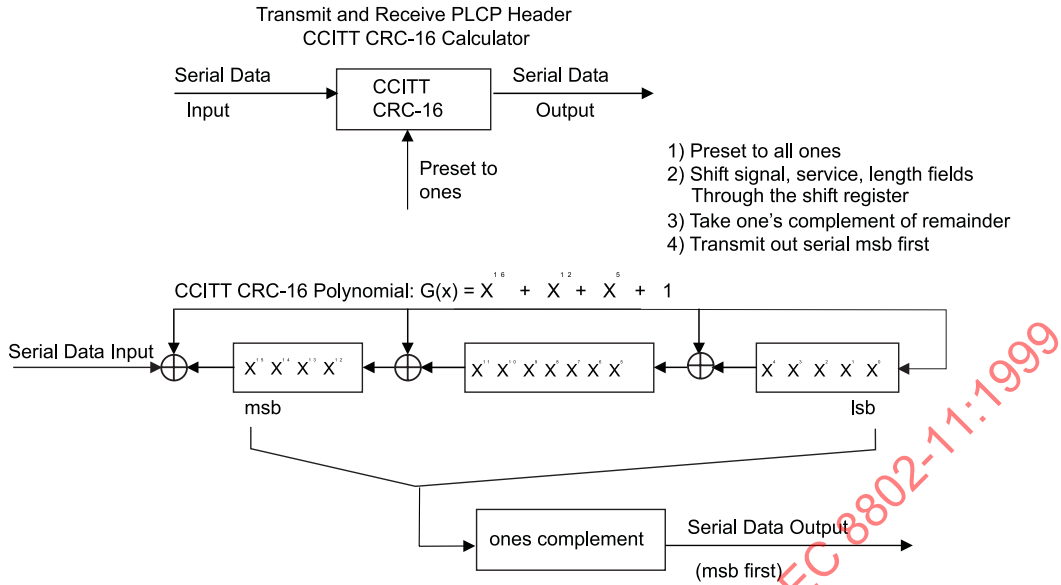
Figure 87—CCITT CRC-16 implementation
