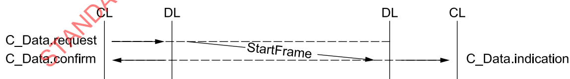
Figure 1 — Example of unsegmented unacknowledged message (known message length)
