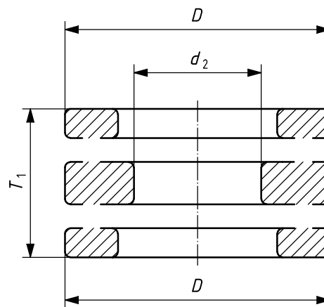
Figure 2 — Double-direction bearings
