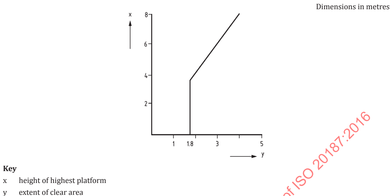
Figure 13 — Clear area around inflatable
