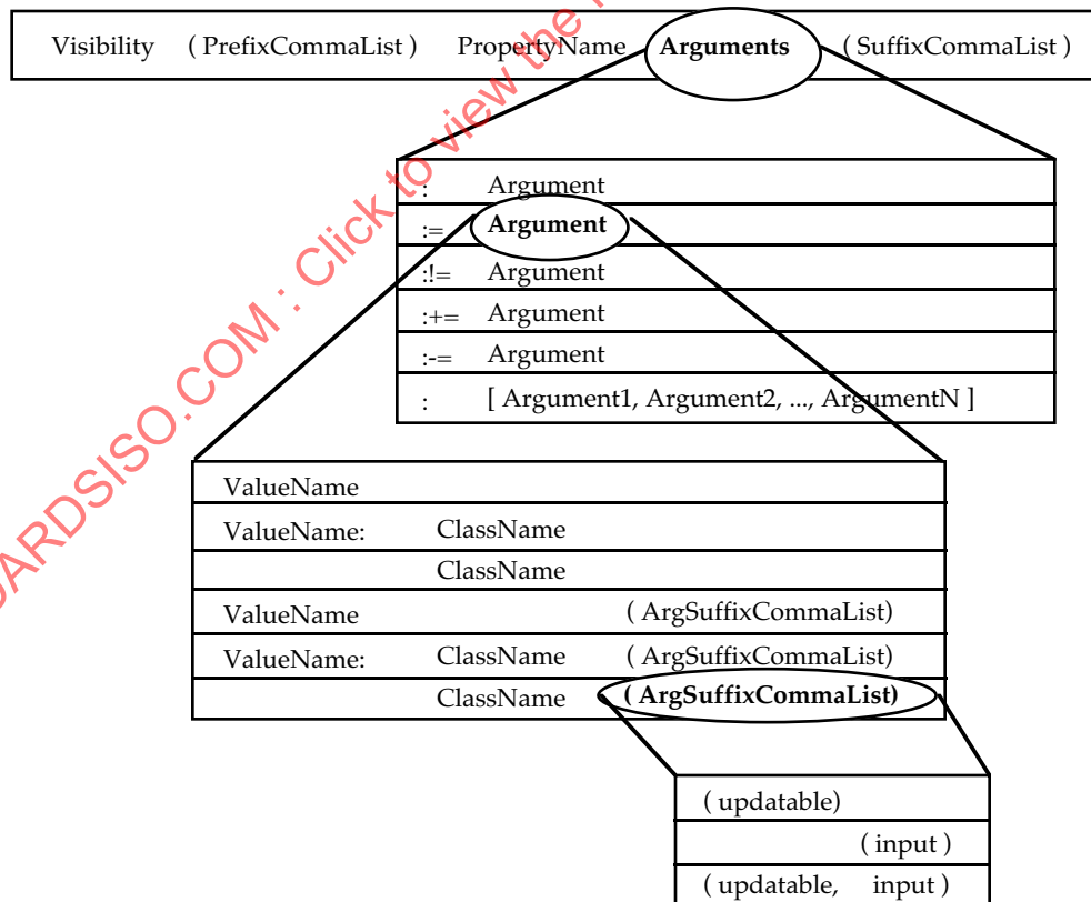
Figure 47—Arguments
