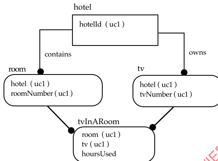
Figure 71—Uniqueness constraints
