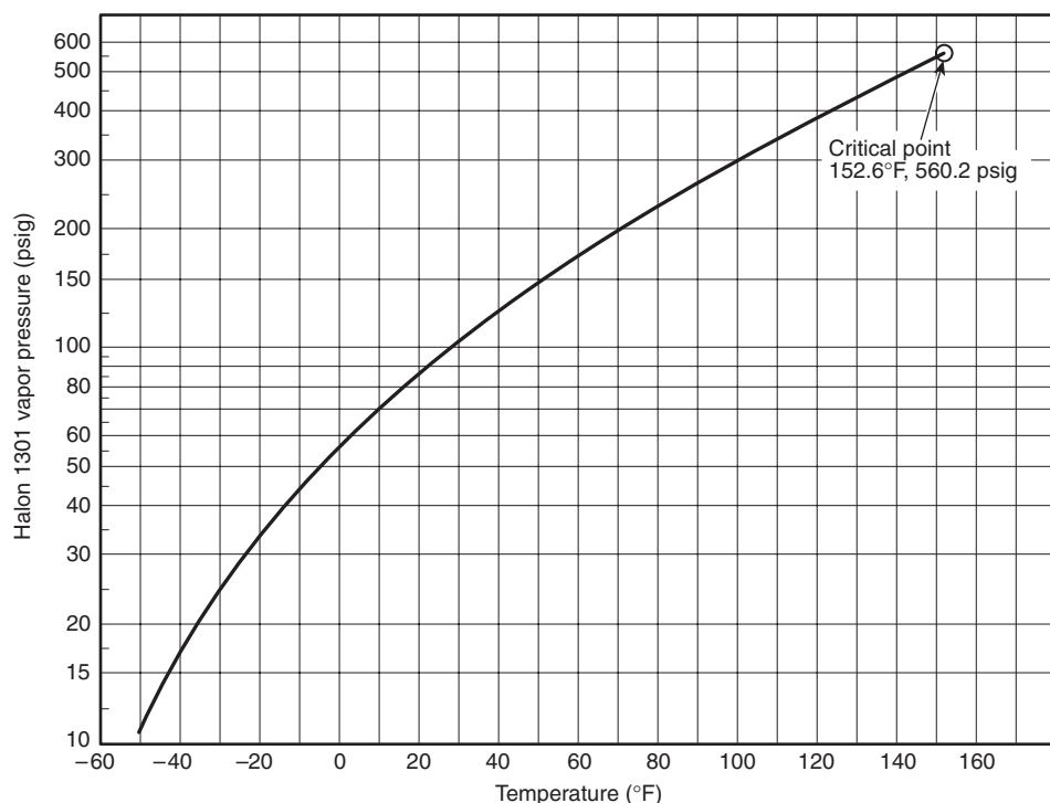
FIGURE C.2.1.1(a) Vapor Pressure of Halon 1301 vs. Temperature.
