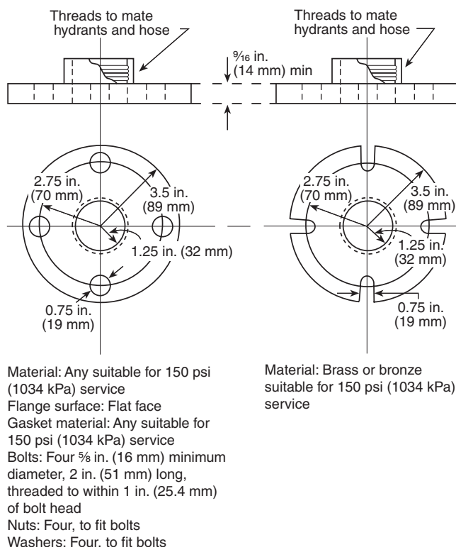
FIGURE 4.13 International Shore Connection.
