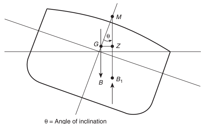
FIGURE 6.7 Center of Buoyancy.
