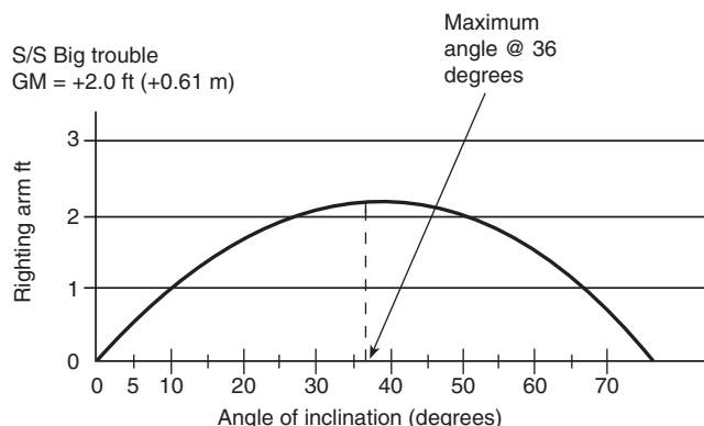
FIGURE 6.8.1 Stability Curve.
