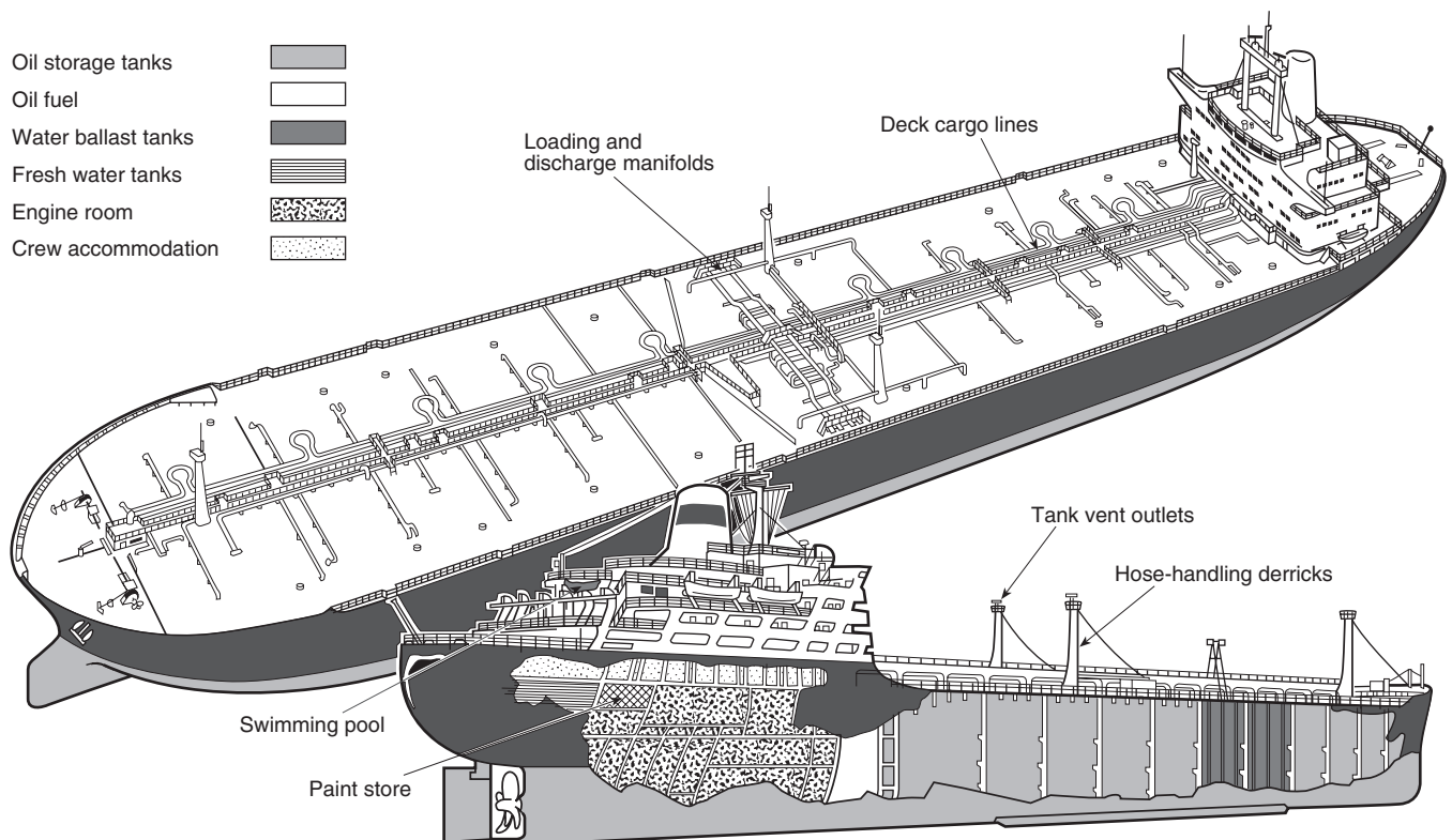
FIGURE 5.3(d) Liquid Bulk Carrier.
