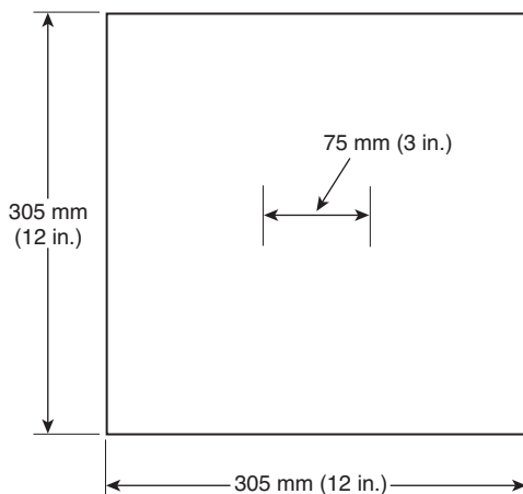
FIGURE 11.3.9.1 Tear Repairs.
