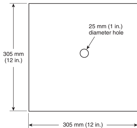
FIGURE 11.3.9.2 Hole Repairs.
