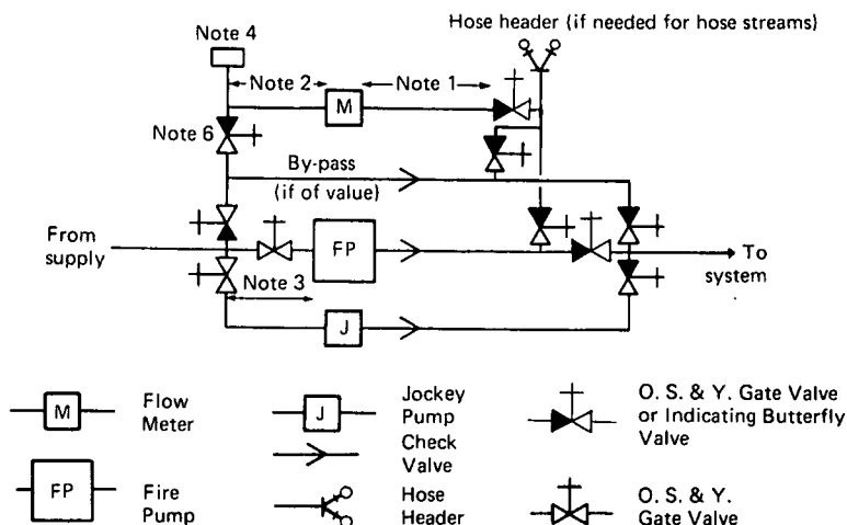
Fig. A-2-13.2.1(b) Diagram of Arrangement for Measuring Fire Pump Water Flow with Meter. Discharge Water Return to Pump Suction. (Not Recommended)
