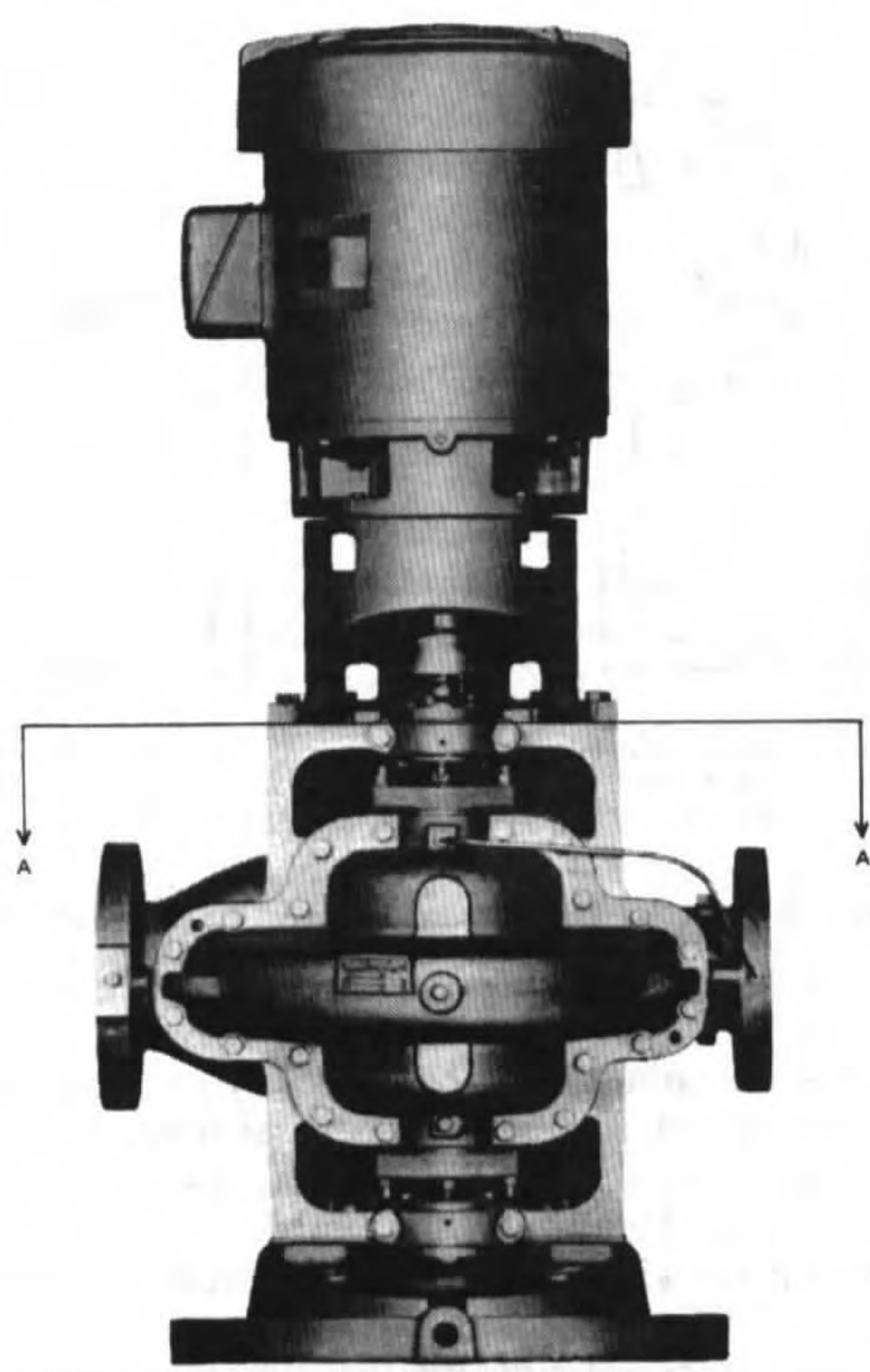
Fig. A-2-16(c) Vertical Pump Shaft Rotation.
