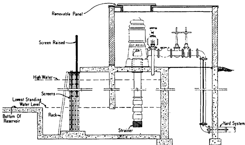
Fig. A-4-2.2.2 Vertical Shaft Turbine-Type Pump — Installation in a Wet Pit.
