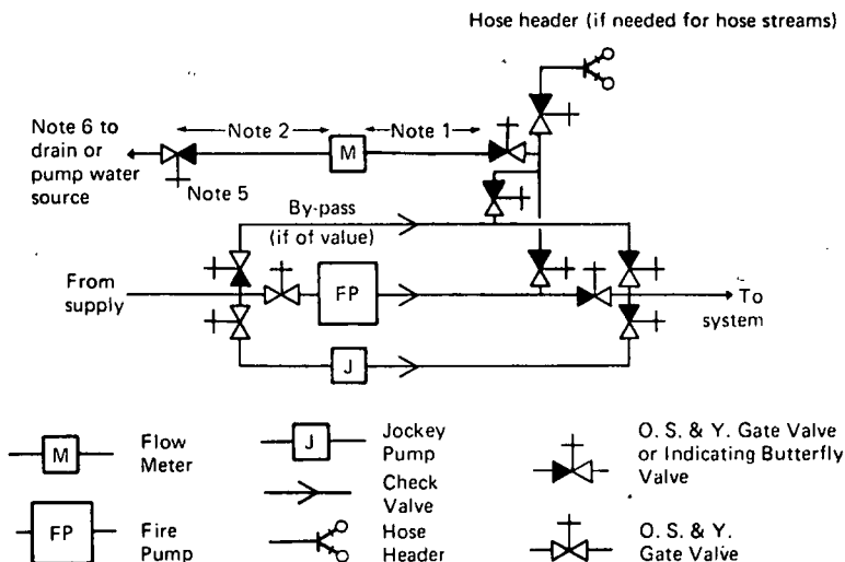
Fig. A-2-13.2.1(a) Diagram of Preferred Arrangement for Measuring Fire Pump Water Flow with Meter. Water Discharge to Drain or to Pump Water Source.
