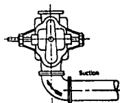
Fig. A-2-9.6 Right and Wrong Pump Suctions.
