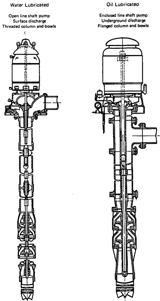
Fig. A-4-1.1 Illustration of Water Lubricated and Oil Lubricated Shaft Pumps.
