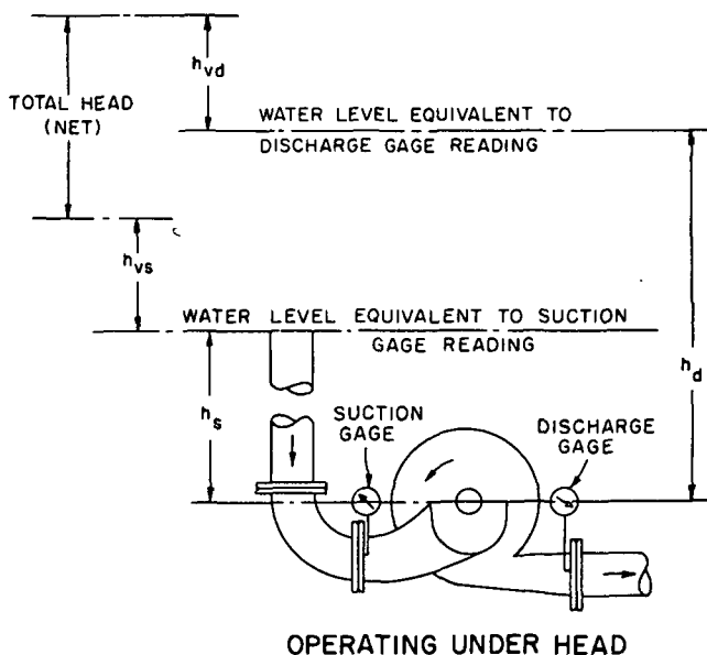
Figure A-1-8.5.7 Typical head of horizontal shaft centrifugal fire pumps.
