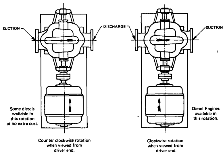
Fig. A-2-16(b) Horizontal Pump Shaft Rotation.
