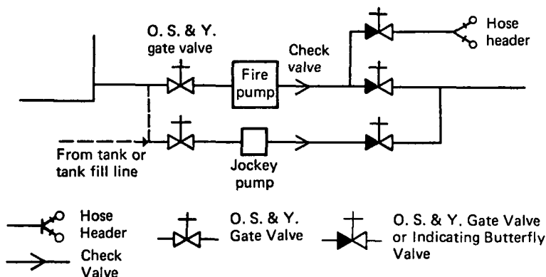
Fig. A-2-19.3 Jockey Pump Installation with Fire Pump.
