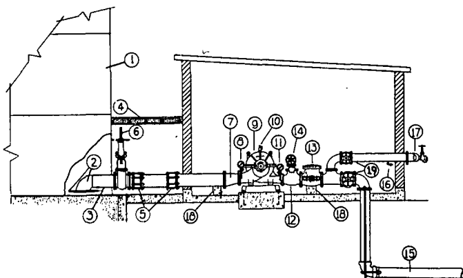
Fig. A-3-3.1 Horizontal Split-Case Fire Pump Installation with Water Supply under a Positive Head.
