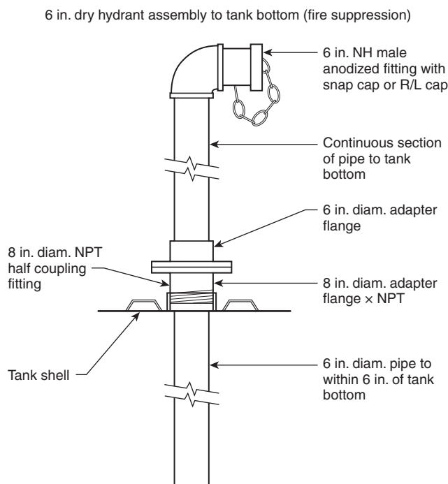
FIGURE A.11.7.4 Typical Dry Hydrant Assembly.
