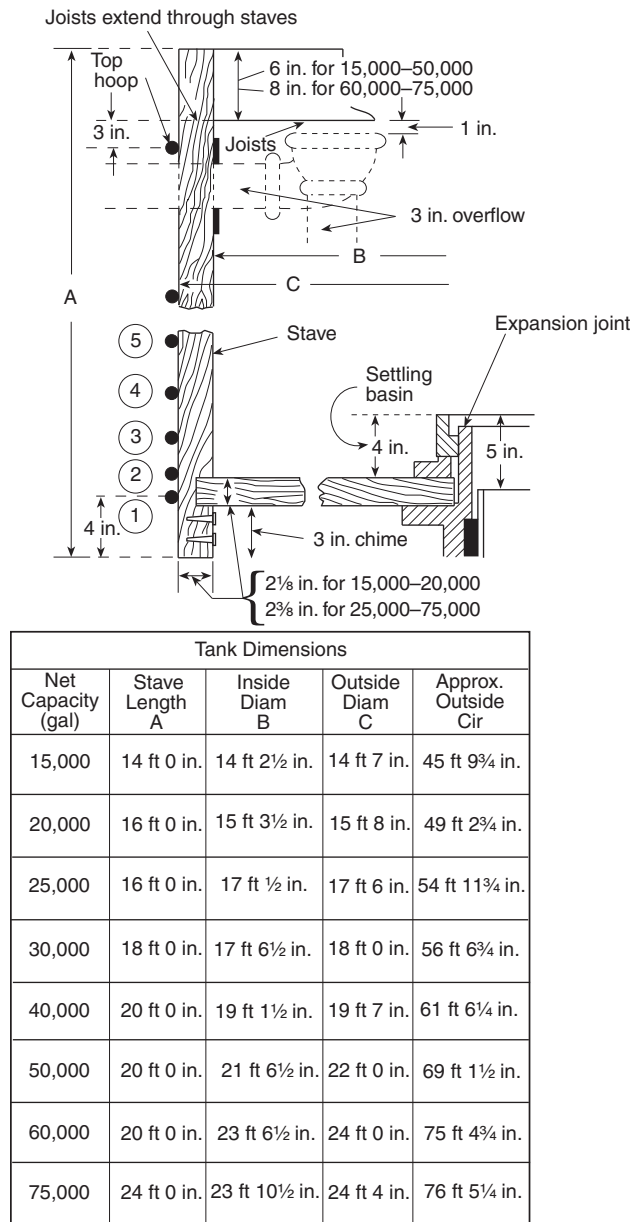
FIGURE A.8.5.3(a) Hoop Schedules for Wood Tanks (dimensions are for cylindrical tanks).
