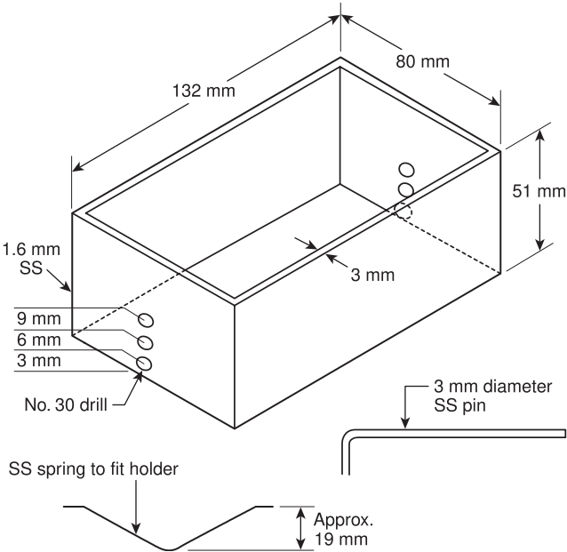
FIGURE 5.9.1 Specimen Holder.
