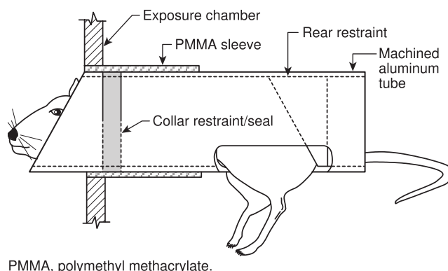
FIGURE A.5.13 Animal Restrainer.
