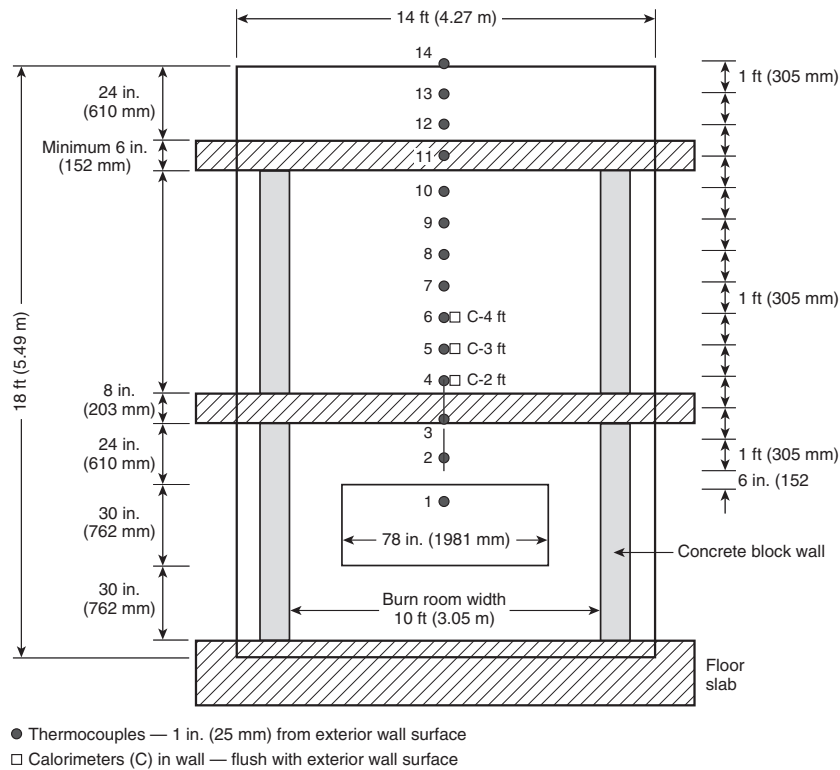
FIGURE 7.1.6(a) Exterior View of the Wall Assembly. Calibration instrumentation (not to scale).
