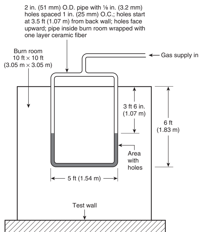
FIGURE 4.4.8 Burn Room Burner — Plan View (not to scale).
