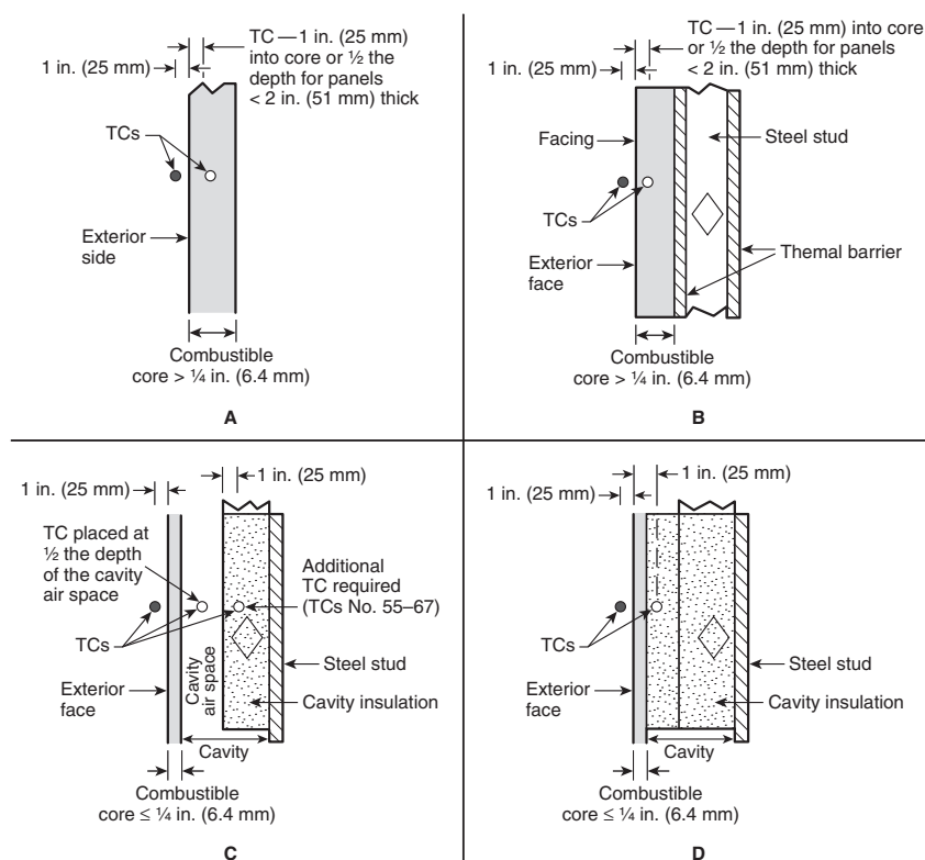
FIGURE 6.1(b) Instrumentation Arrangement.
