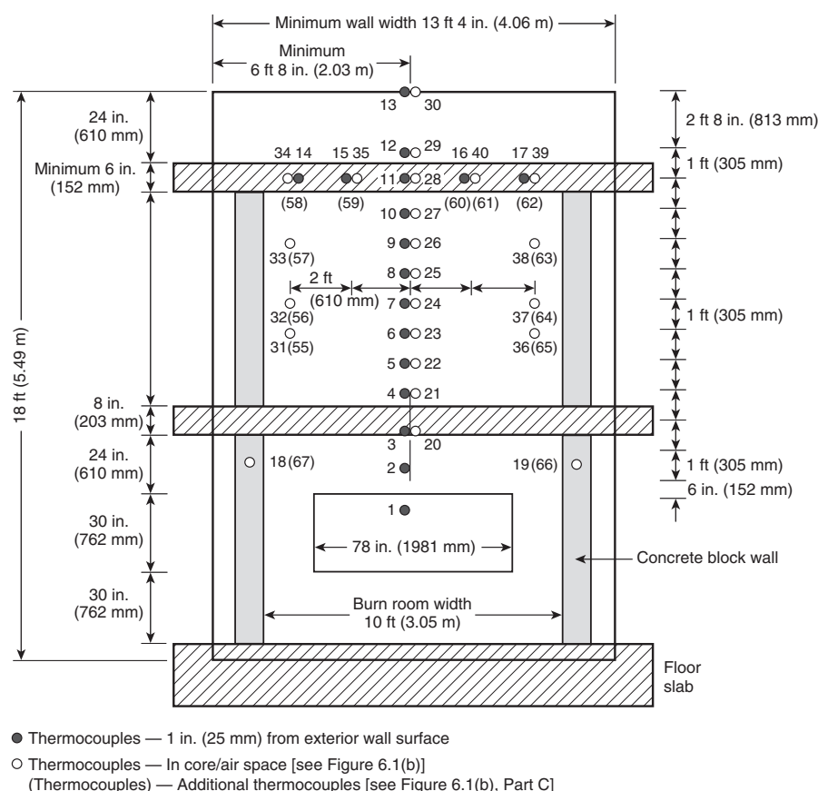
FIGURE 6.1(a) Exterior Face of the Test Specimen. Instrumentation arrangement.
