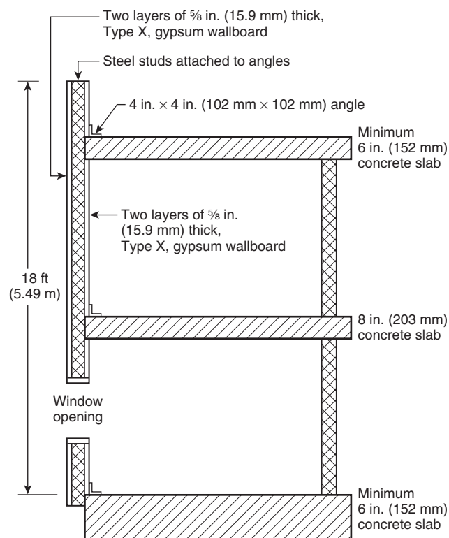
FIGURE A.7.1.1 Side View of Calibration Wall Assembly (not to scale).
