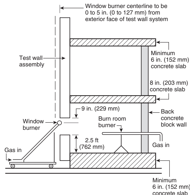
FIGURE A.4.4.8 Side View of Burner Placement in First-Story Test Room (not to scale).
