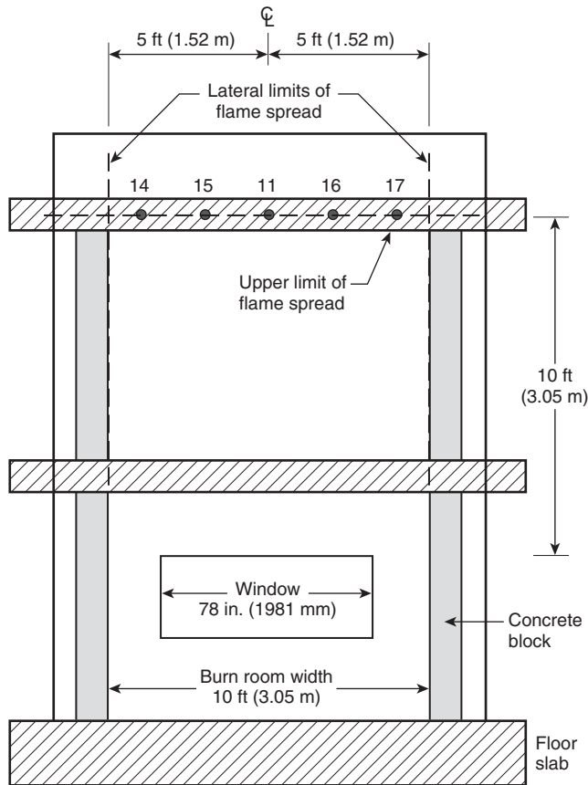
FIGURE 10.2.1.2 Limits of Flame Propagation (not to scale).
