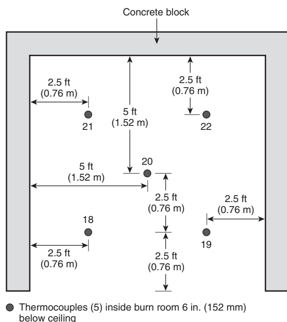
FIGURE 7.1.6(c) Plan View — First-Story Test Room. Calibration instrumentation (not to scale).
