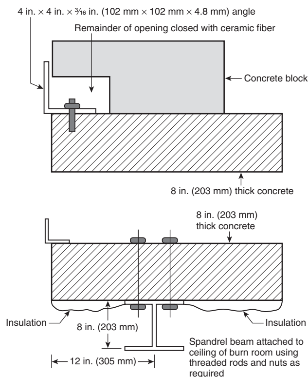
FIGURE A.4.2.3(c) Side View of Burner Placement in First-Story Test Room (not to scale).
