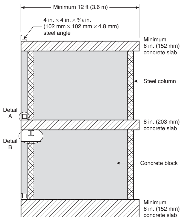
FIGURE A.4.2.3(b) Plan View of Test Apparatus — Both Floors (not to scale).
