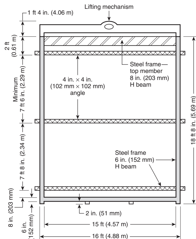
FIGURE 4.3.1.3 Front View of Movable Wall Frame (not to scale).
