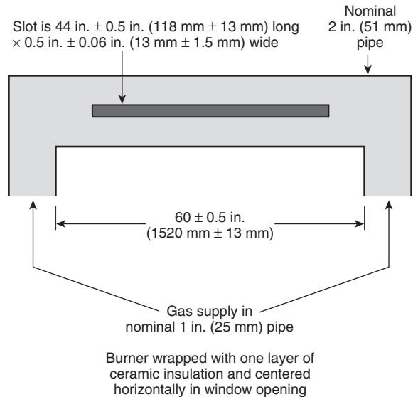
FIGURE 4.4.11 Plan View of Window Burner (not to scale).
