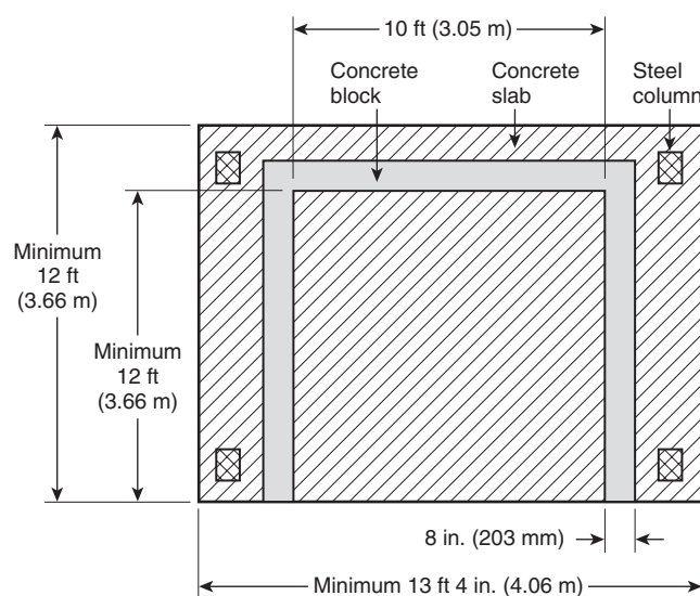
FIGURE A.4.2.3(a) Front View of Test Apparatus (not to scale).
