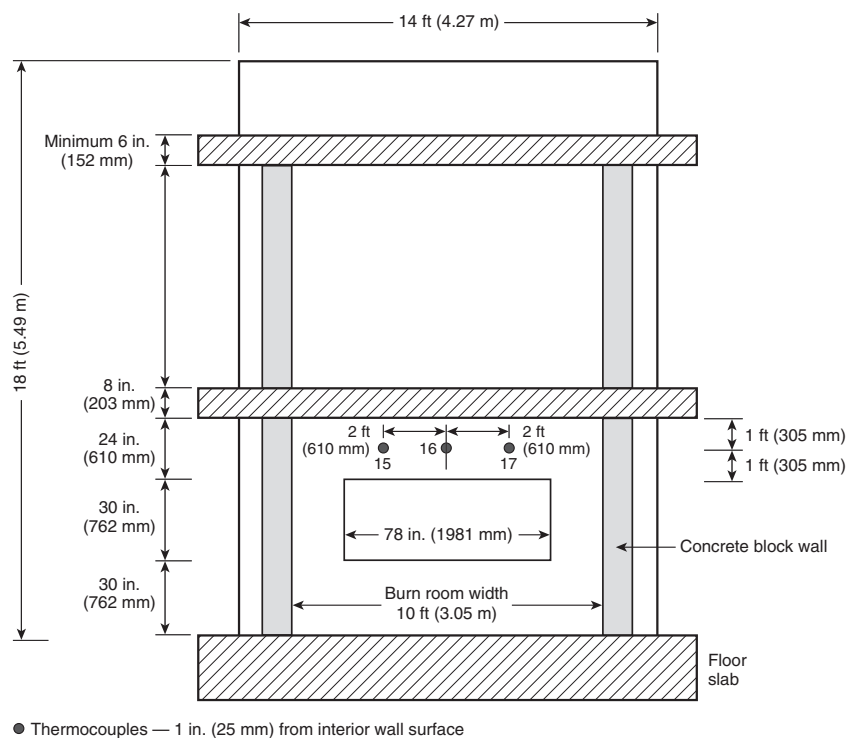
FIGURE 7.1.6(b) Interior View of the Wall Assembly. Calibration instrumentation (not to scale).
