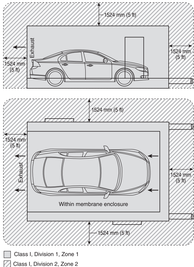
N FIGURE 14.4.6.4 Electrical Classifications for Inflatable Finishing Workstations.
