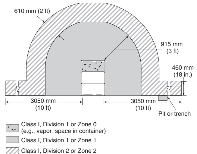
FIGURE 6.6.2 Electrical Area Classification Around an Open Container in a Ventilated Area.
