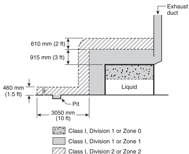
FIGURE 6.4(c) Electrical Area Classification for Open Dipping and Coating Processes with Partial Peripheral Vapor Containment and Ventilation — Vapors NOT Confined to Process Equipment.
