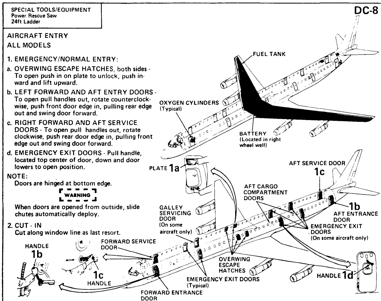
Figure A-22 Douglas DC-8.
