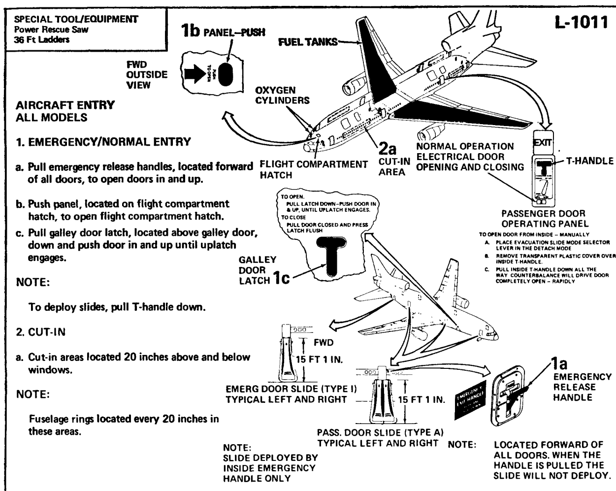
Figure A-27 Lockheed L-1011 "Wide Body."
