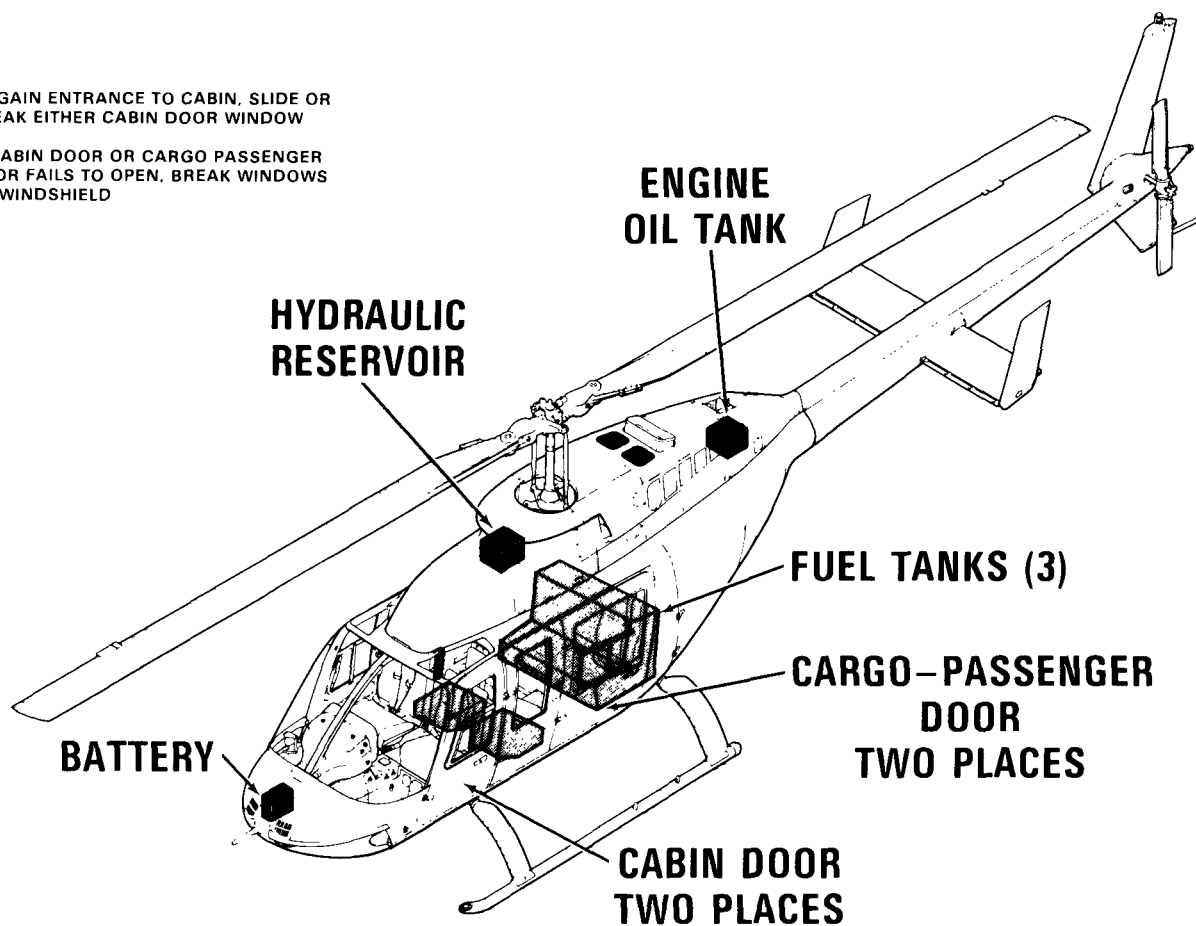
Figure A-6 Bell 206L helicopter.
