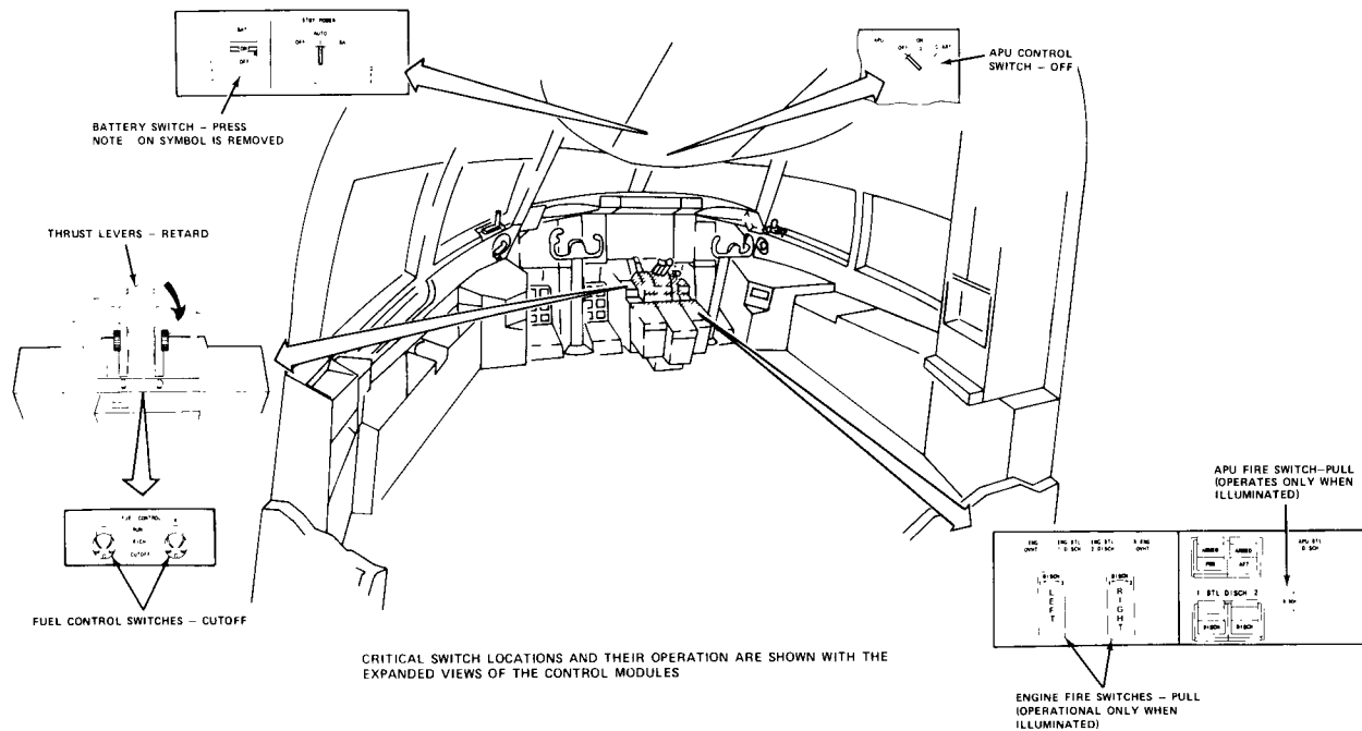
Figure A-32 Boeing 767 cockpit control switch locations.
