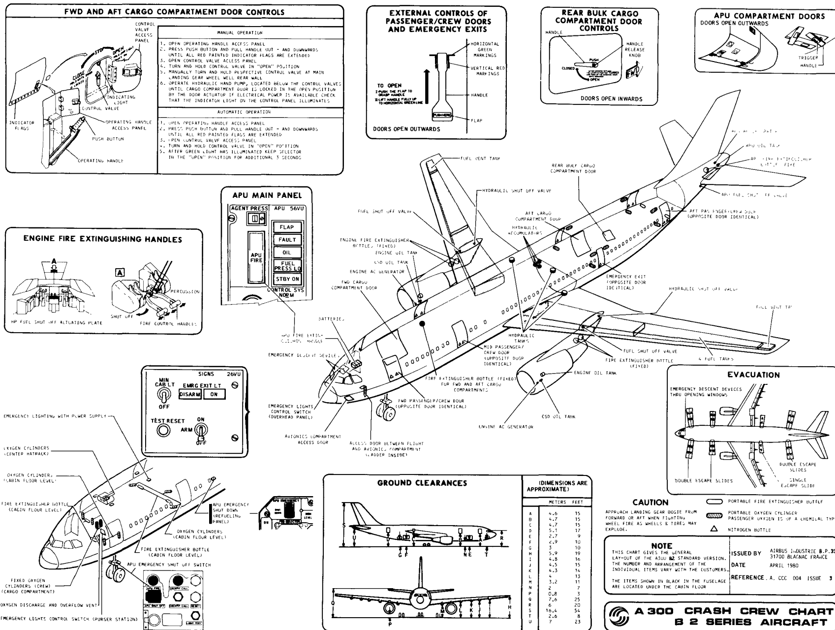
Figure A-43 Airbus Industrie A300 crash crew chart, B2 series aircraft.
