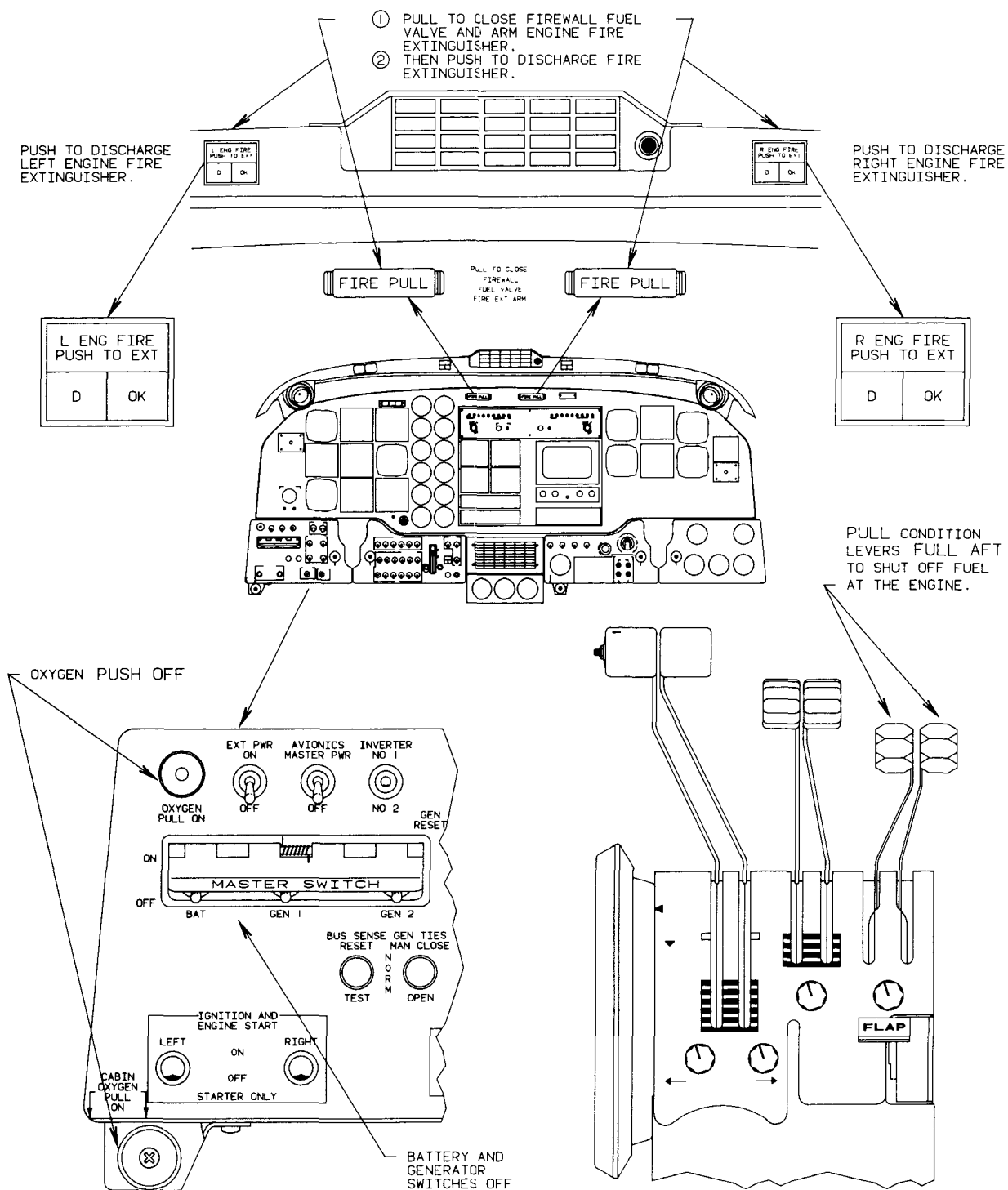
Figure A-31(b) Beech Model 1900.
