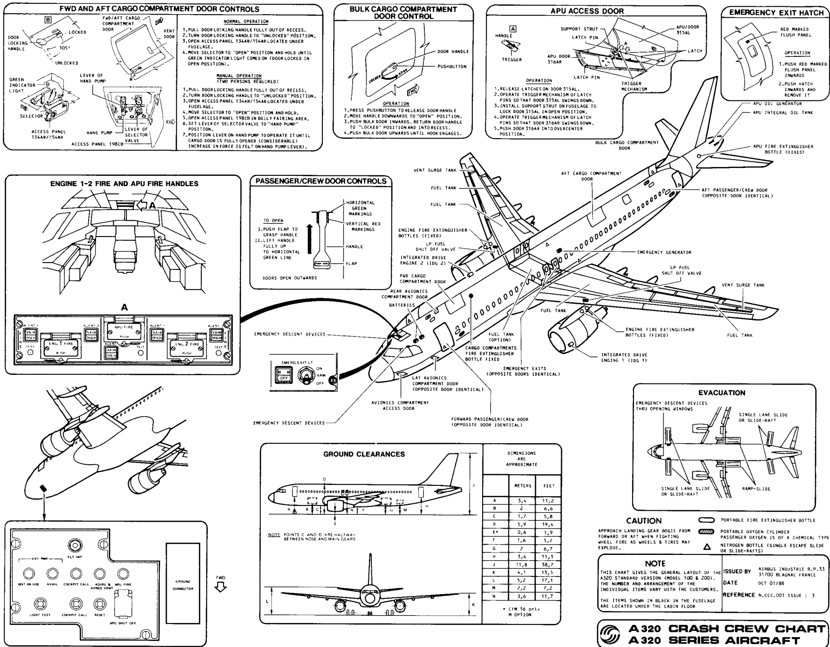
Figure A-46 Airbus Industrie A320 crash crew chart, A320 series aircraft.
