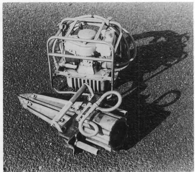
Figure 7-4(d) Hydraulic rescue tool. This portable tool is capable of applying extreme pressures to spread, cut, and lift. It can provide valuable forcible entry application in aircraft accident operations.
