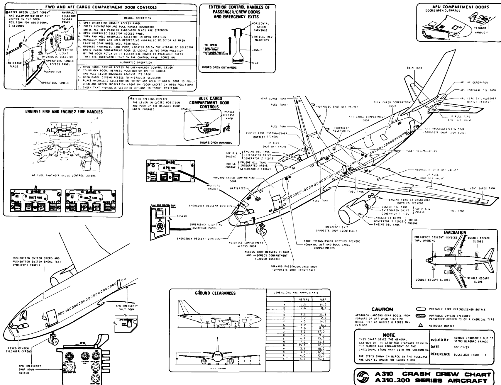
Figure A-42 Airbus Industrie A310 crash crew chart, A310-300 series aircraft.
