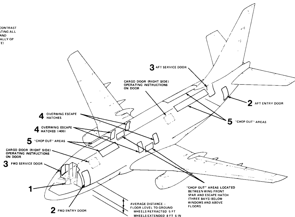
Figure A-38 Boeing 737 emergency rescue access.
