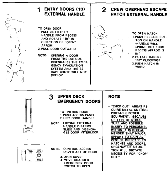
Figure A-36(b) Boeing 747 emergency rescue access.
