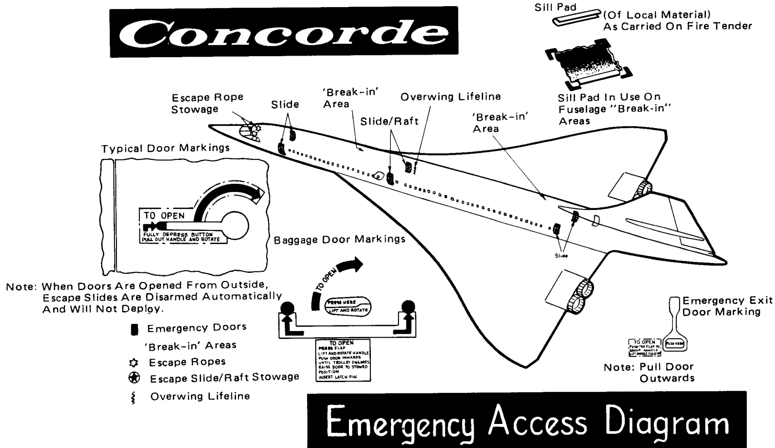
Figure A-17 Concorde.
