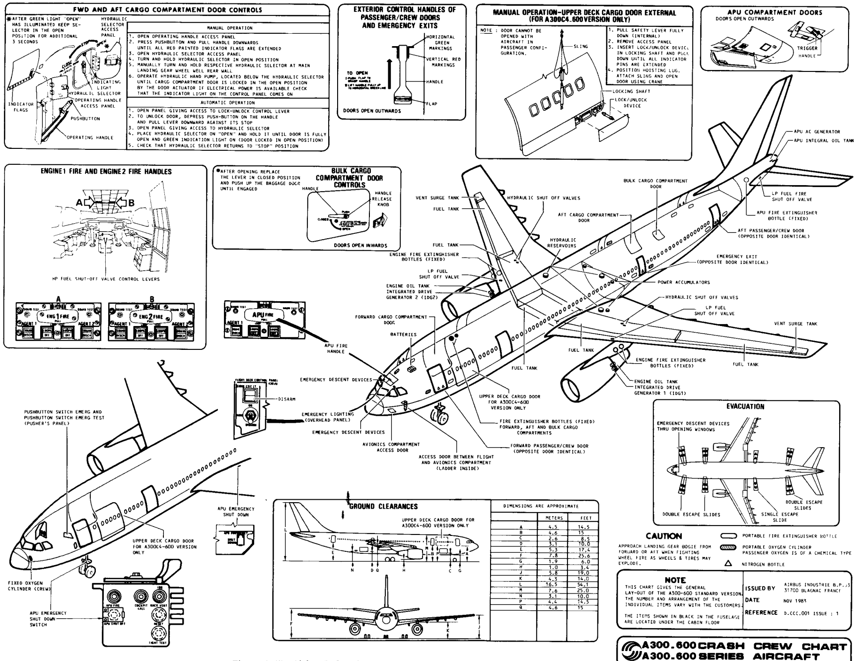
Figure A-45 Airbus Industrie A300-600 crash crew chart, A300-600 series aircraft.
