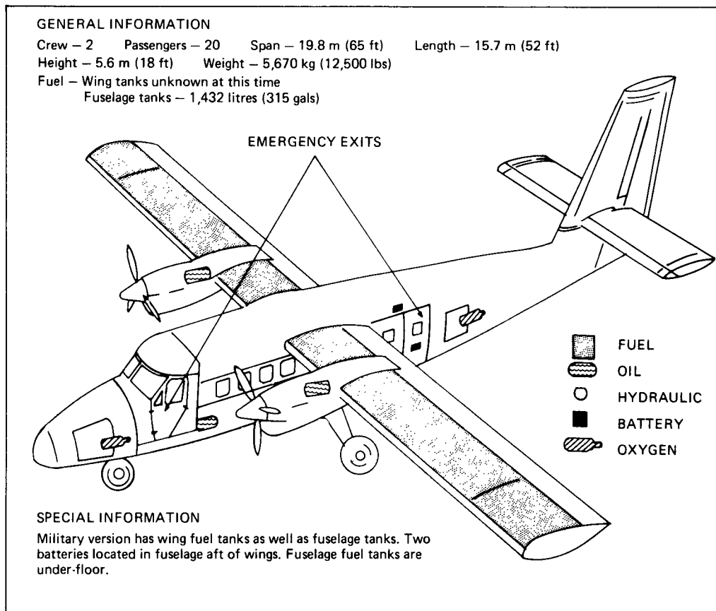
Figure A-19 DeHaviland Twin Otter.
