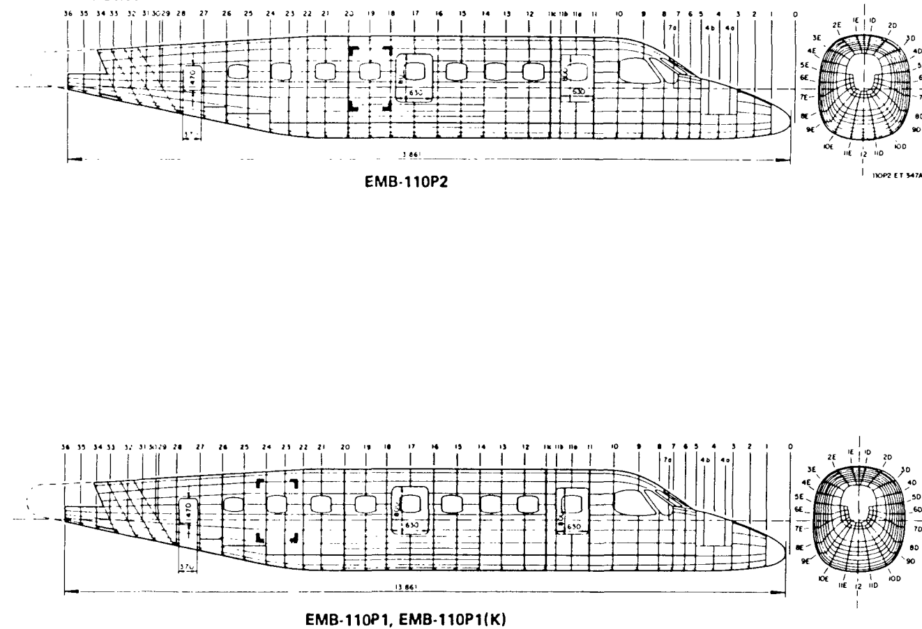
Figure A-49 Embraer EMB-110P2, EMB-110P1, and EMB-110P1(K) break-in points.
