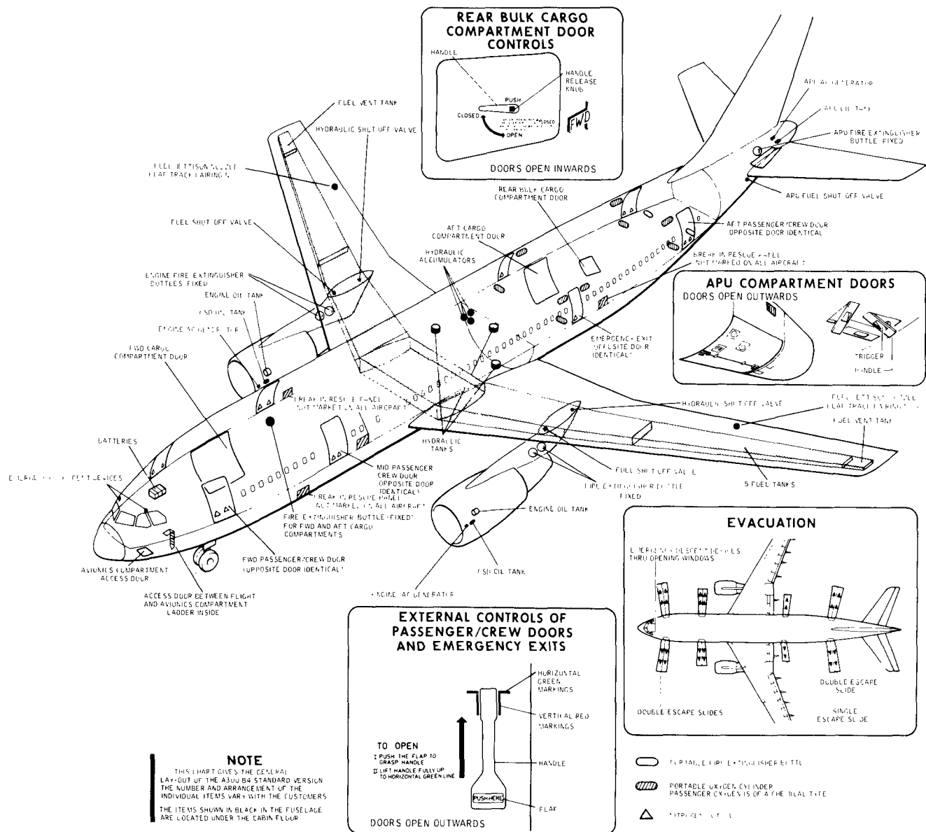
Figure A-29 A-300 Air Bus "Wide Body."
