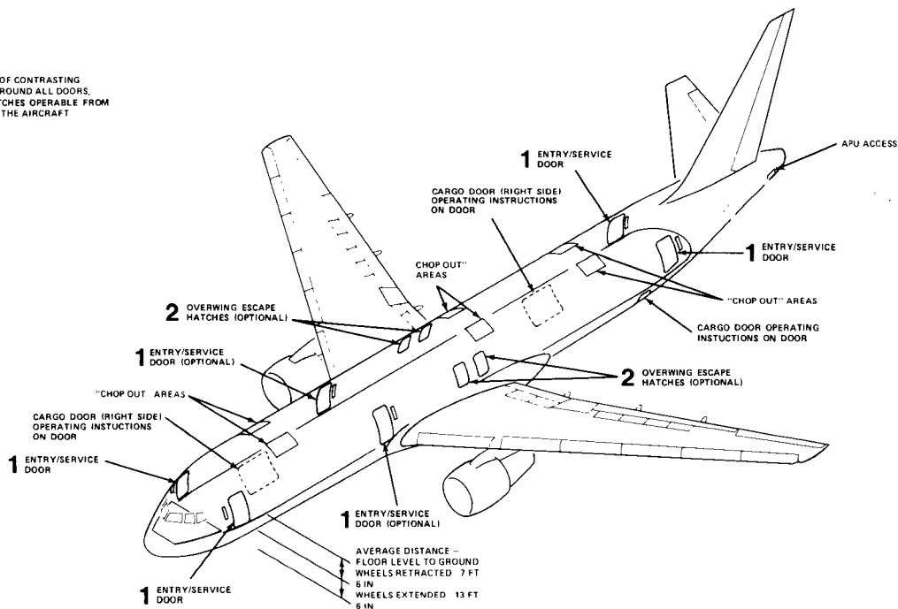
Figure A-33(a) Boeing 767 emergency rescue access.
