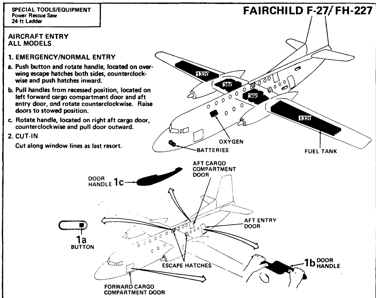
Figure A-26 Fairchild F-27.
