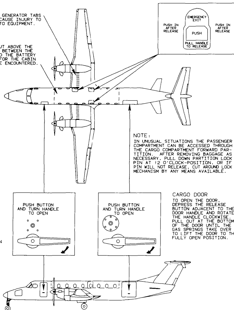
Figure A-31(a) Beech Model 1900.
