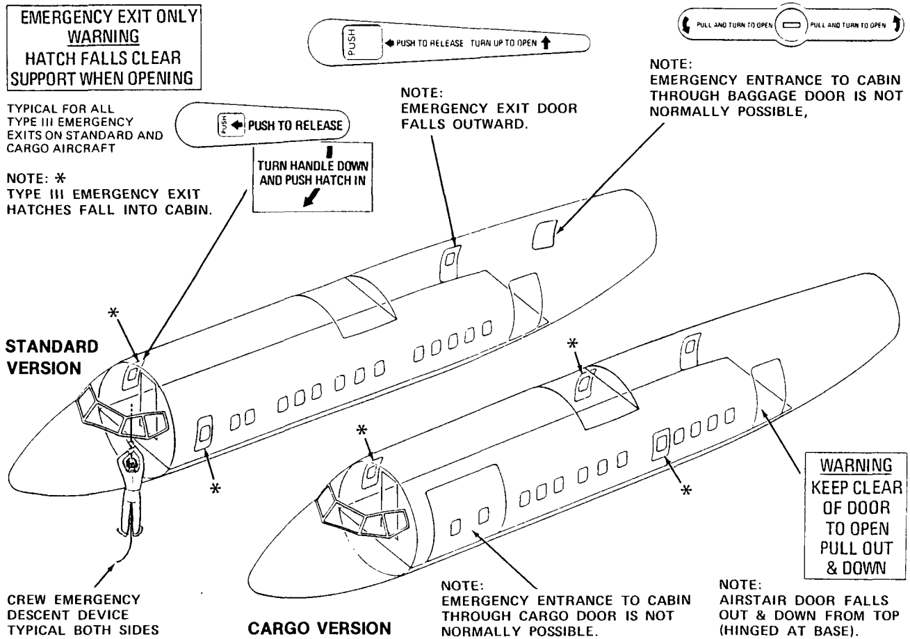
Figure A-18 DeHaviland Dash 7.
