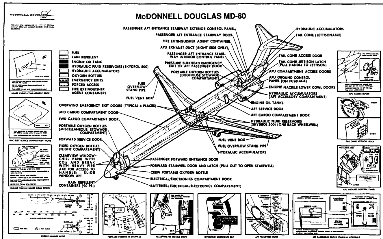
Figure A-24 McDonnell Douglas MD-80.
