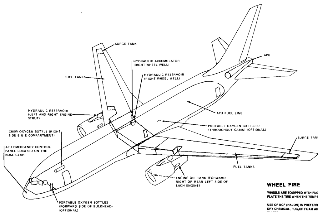
Figure A-34 Boeing 767 flammable material locations.
