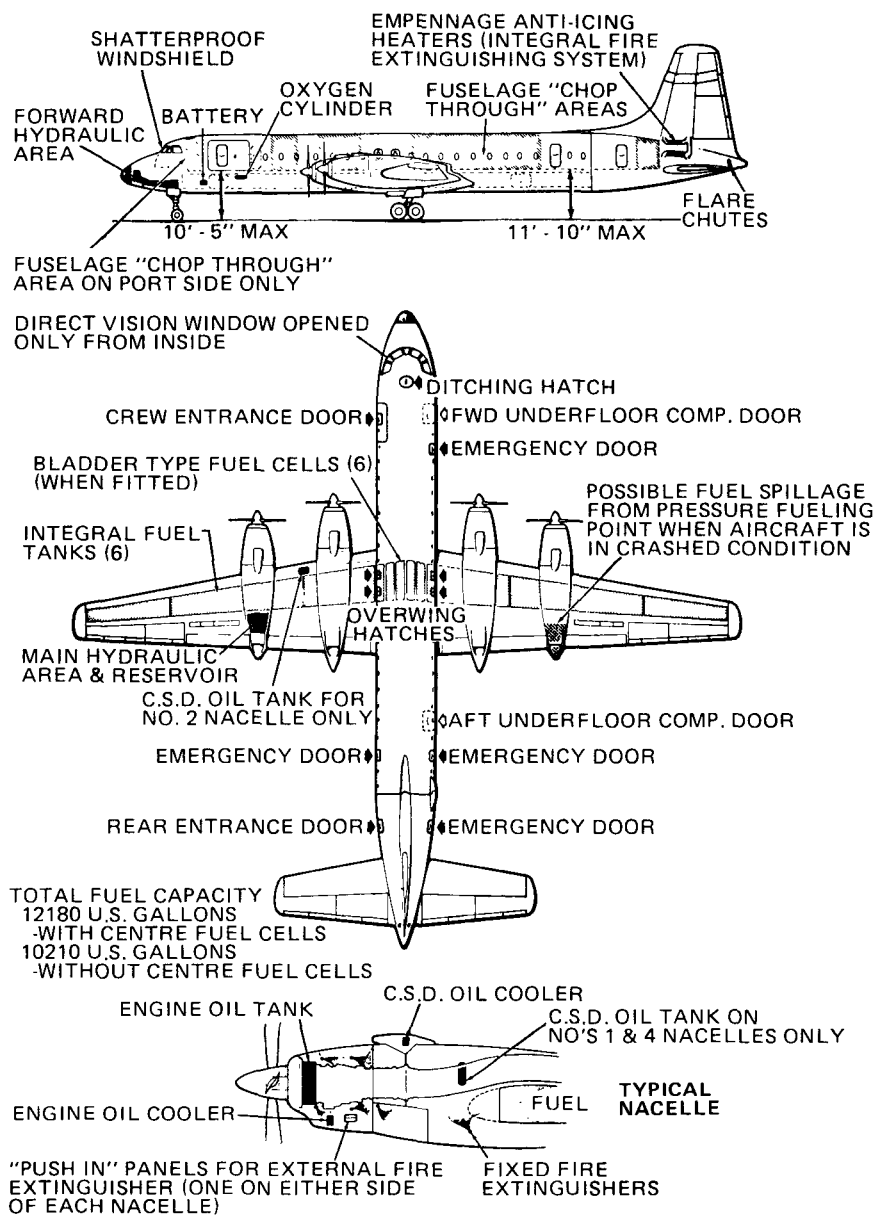
Figure A-14 Canadair CL-44D4 cargo/passenger aircraft.
