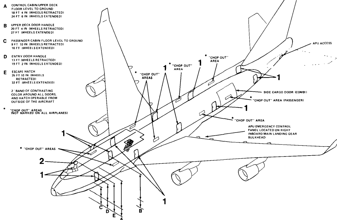
Figure A-36(a) Boeing 747 emergency rescue access.
