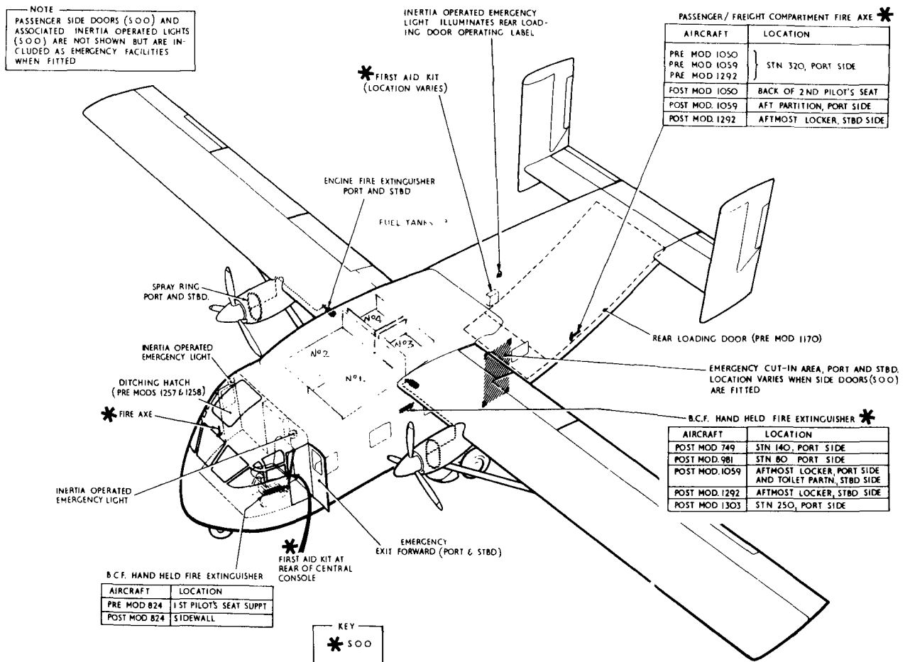
Figure A-28 Short Dash 80.
