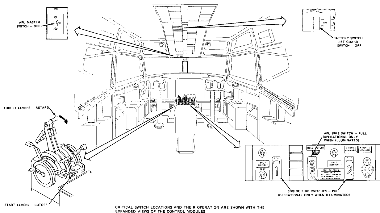
Figure A-39 Boeing 737 cockpit control switch locations.
