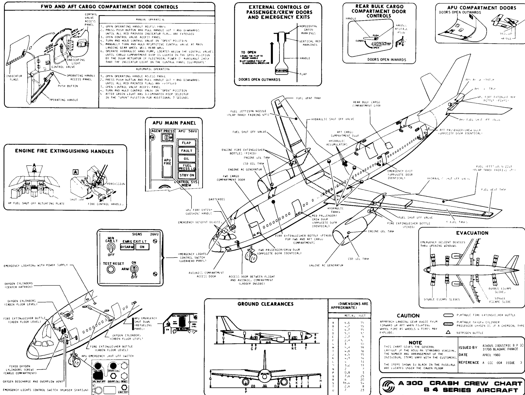
Figure A-47 Airbus Industrie A300 crash crew chart, B4 series aircraft.
