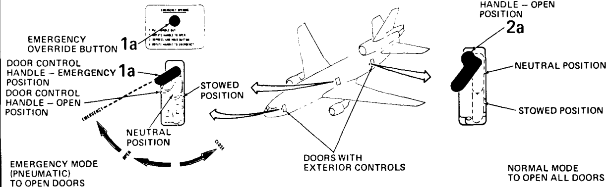
Figure A-25 Douglas DC-10 "Wide Body."
