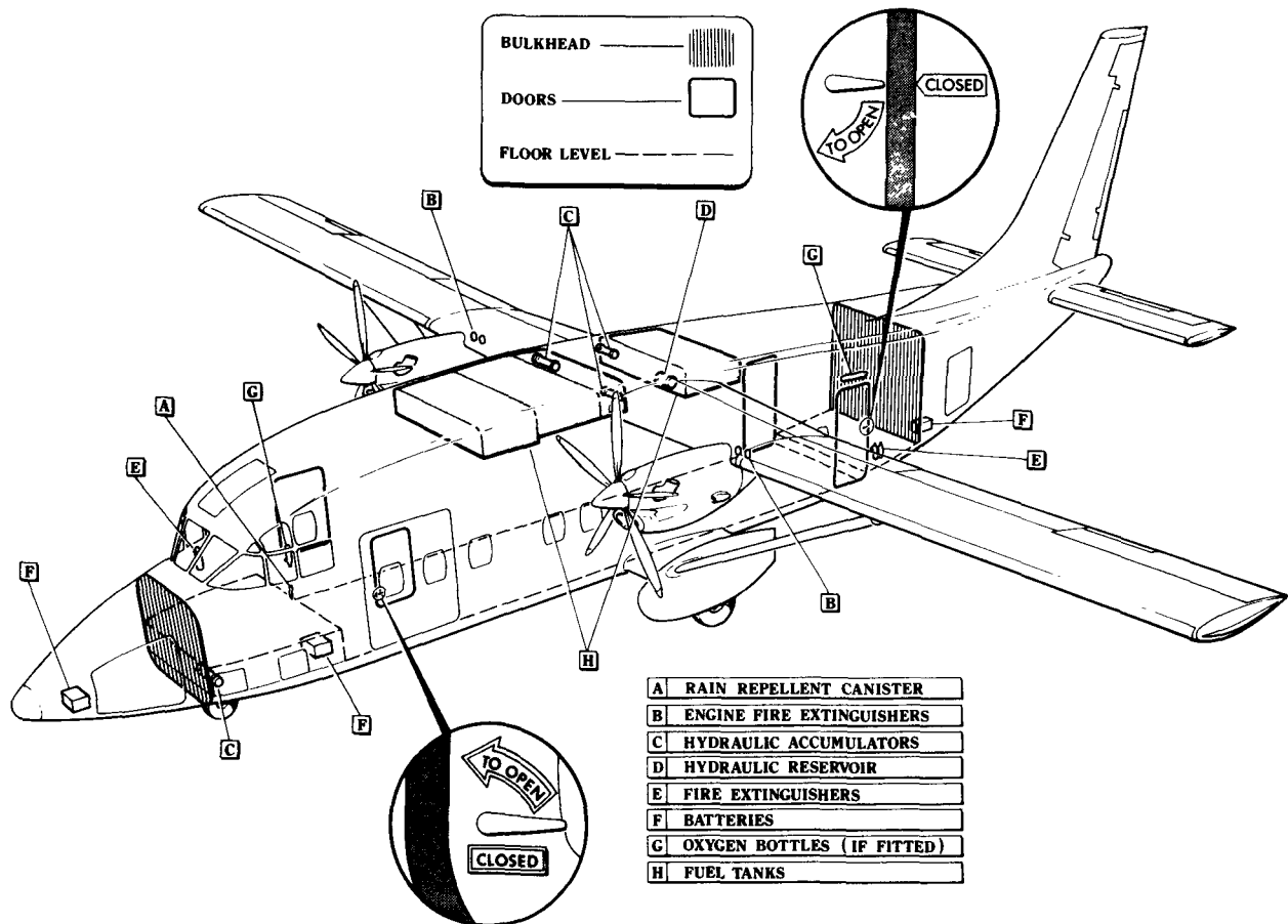
Figure A-30 Shorts SD 3.60.
