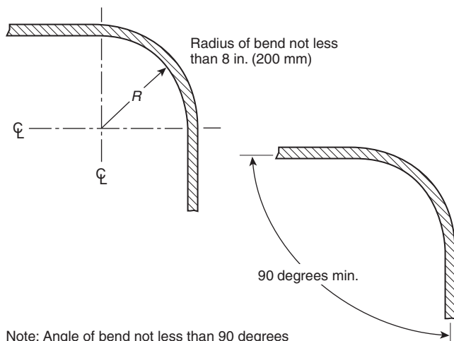
FIGURE 4.9.5 Conductor Bends.
