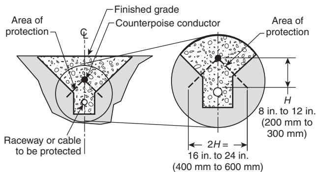
FIGURE A.11.4.2.6.1.6 Area of Protection.
