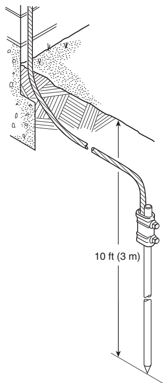
FIGURE 4.13.2.3.1 Typical Single Ground Rod Installation.
