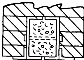
Figure 16. Steel lintel.
