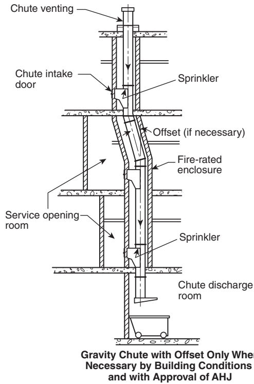
FIGURE A.5.2(b) Gravity Waste Chute.
