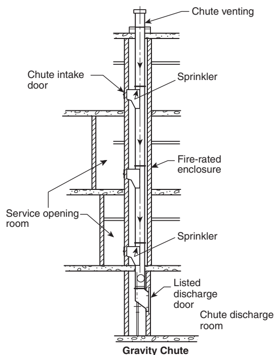
FIGURE A.5.2(a) Gravity Linen Chute.
