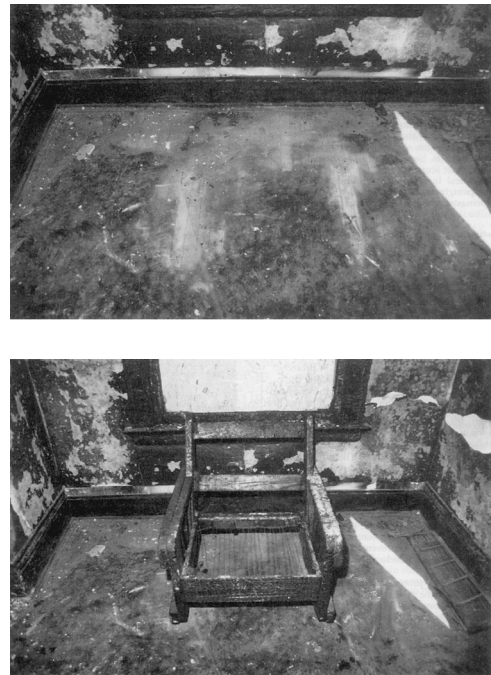
FIGURE 6.15.2.1 Photograph on Top, Showing Protected Area; Photograph at Bottom, Showing How the Chair Was Positioned During the Fire.
