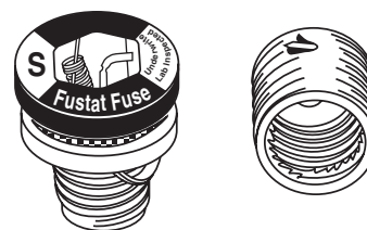
FIGURE 8.6.2.1.1(c) A Type S Nonrenewable Fuse and Adapter. The Time-Lag Type of Fuse is Acceptable But Not Required.
