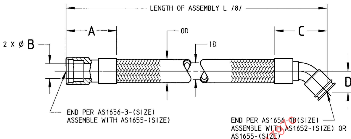
FIGURE 1 - HOSE ASSEMBLY
