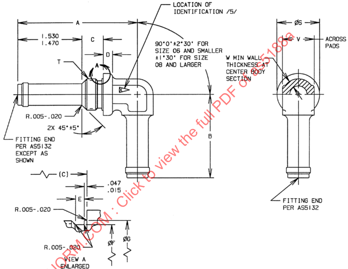
FIGURE 1 - FITTING, ELBOW, 90°
