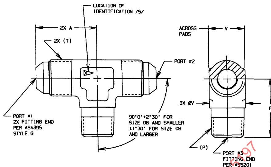
FIGURE 1 - FITTING, TEE
