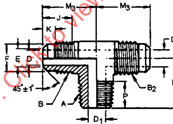
FIGURE 34—TWO-WAY REDUCING TEE (100425) (T1)
