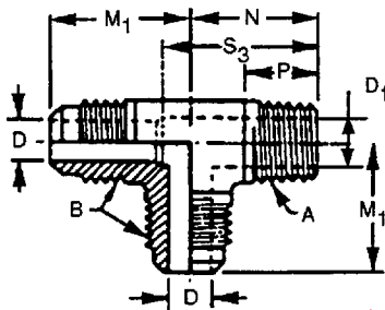
FIGURE 19—RIGHT ANGLE TWO-WAY TEE (010424) (T3)
