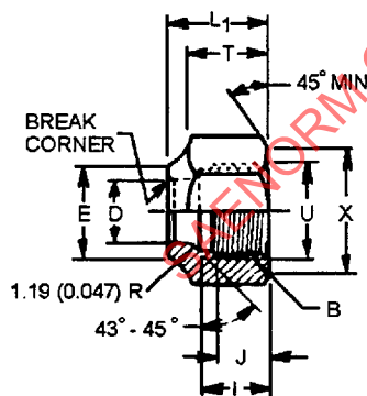
FIGURE 36A—SHORT NUTS (010166) (NS4)
