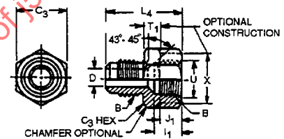
(R) FIGURE 6—INTERNAL FLARE TO EXTERNAL FLARE ADAPTER (010105) (UR3)
