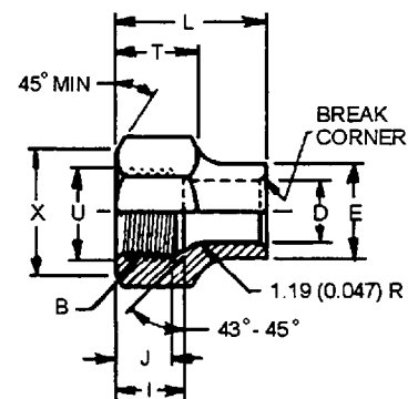
FIGURE 36B—LONG NUTS (010167) (N4)
