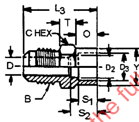
FIGURE 2—FUSIBLE CONNECTOR (HALF UNION) (010163) (FU)
