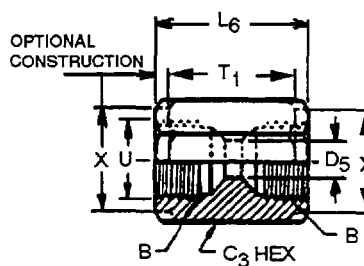
(R) FIGURE 8—INTERNAL FLARE UNION (010107) (U4)
