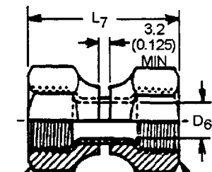
(R) FIGURE 6—INTERNAL FLARE TO EXTERNAL FLARE ADAPTER (010105) (UR3)
