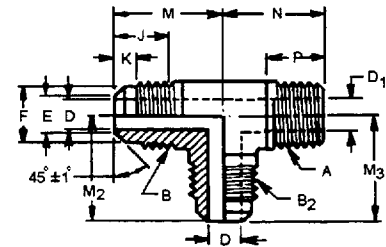
FIGURE 35—RIGHT ANGLE TWO-WAY REDUCING TEE (1010424) (T3)
