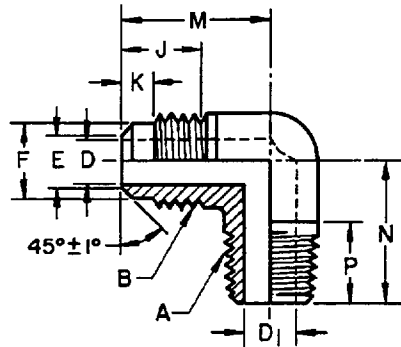
FIGURE 11—90 DEGREE ELBOW (010202) (E1)
