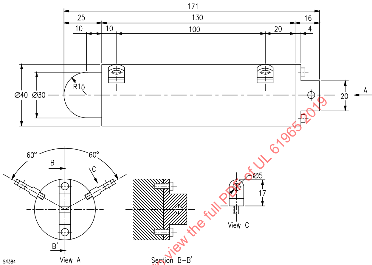
Figure 11 Example of 1,4 kg steel missile
