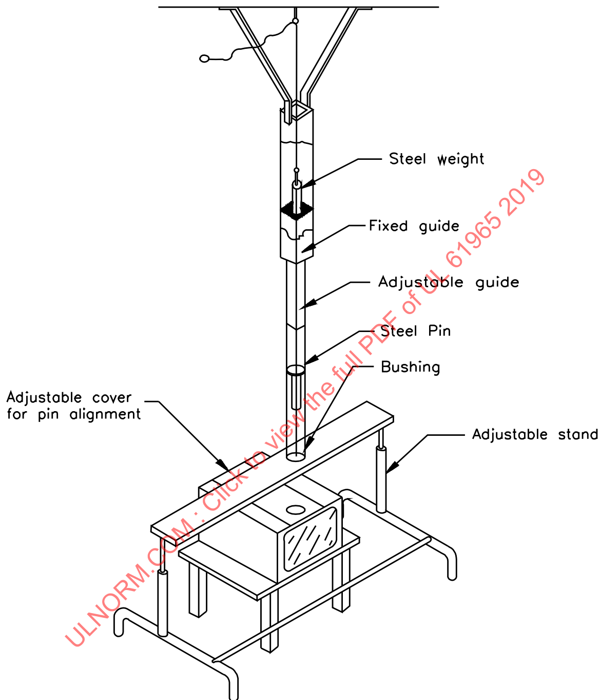
Figure 8 Example of high-energy impact test set-up
