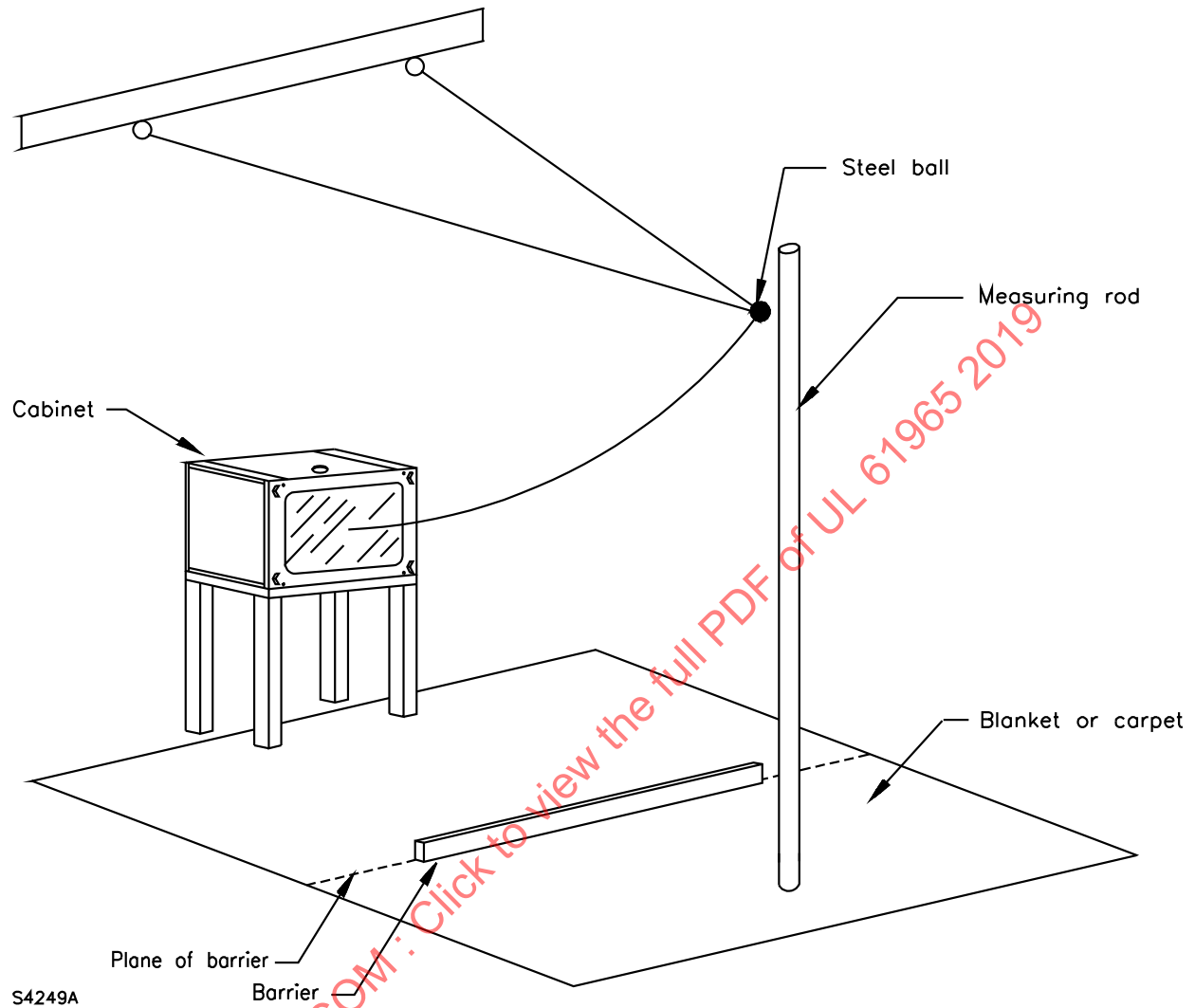
Figure 2 Example of a ball impact test
