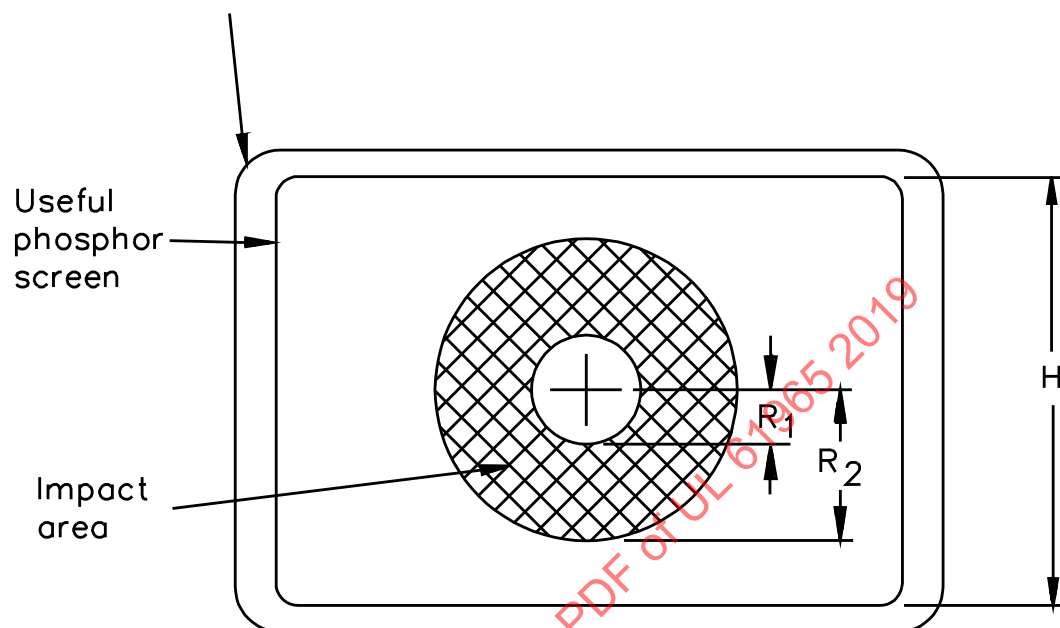
Figure 4 Missile impact area on a typical CRT Glass envelope
