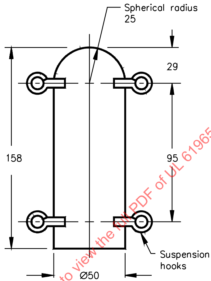
Figure 3 Example of a 2,3 kg steel missile
